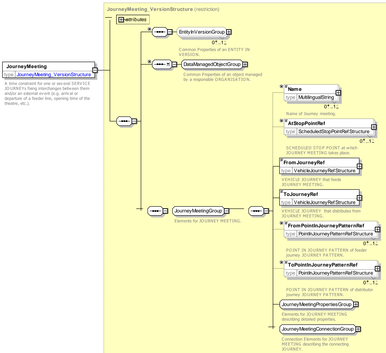
Figure 100 — JourneyMeeting — XSD
