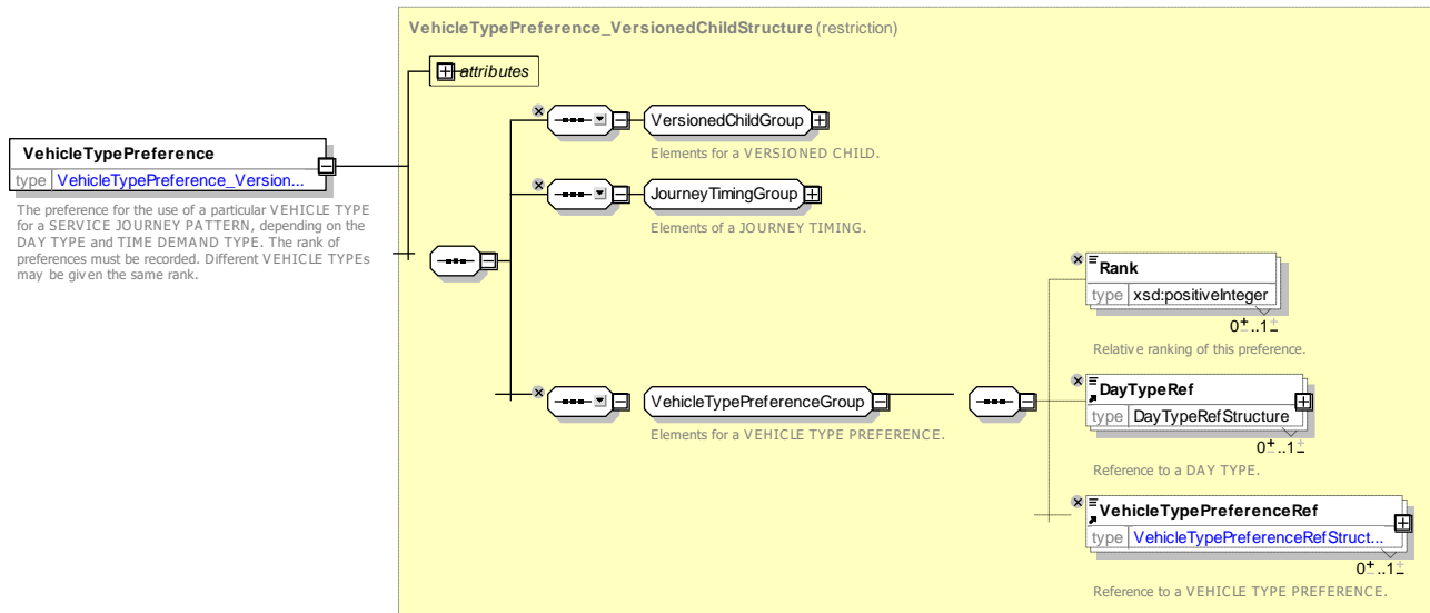
Figure 76 — VehicleTypePreference — XSD
