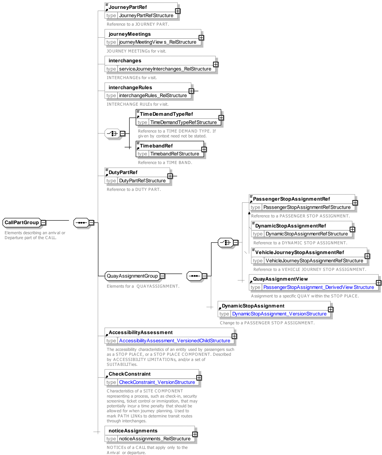
Figure 159 — CallPartGroup — XSD
