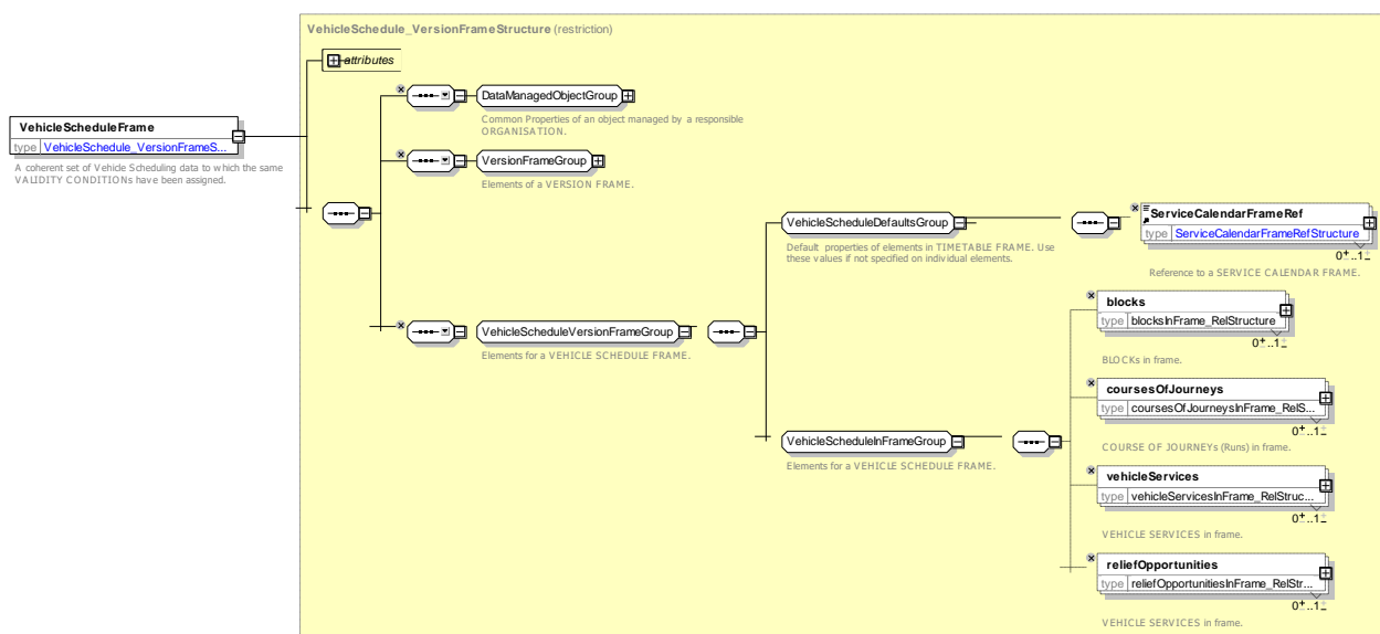
Figure 171 — VehicleScheduleFrame — XSD
