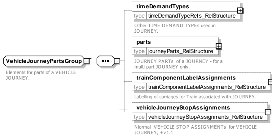
Figure 19 — VehicleJourneyPartsGroup — XSD
