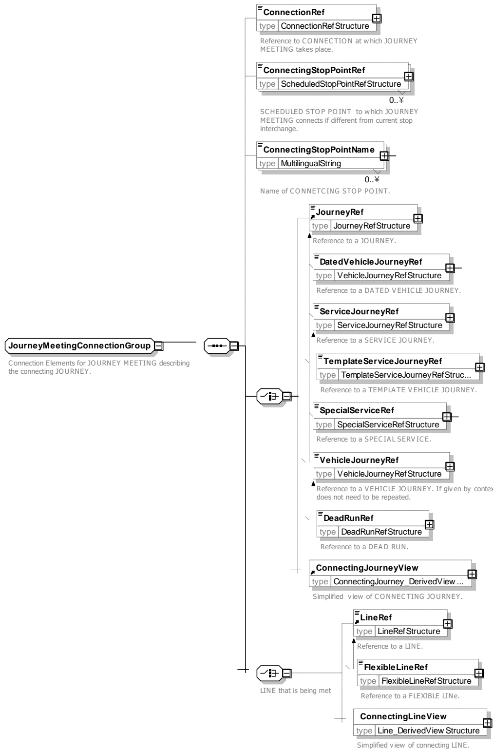
Figure 102 — JourneyMeetingConnectionGroup — XSD
