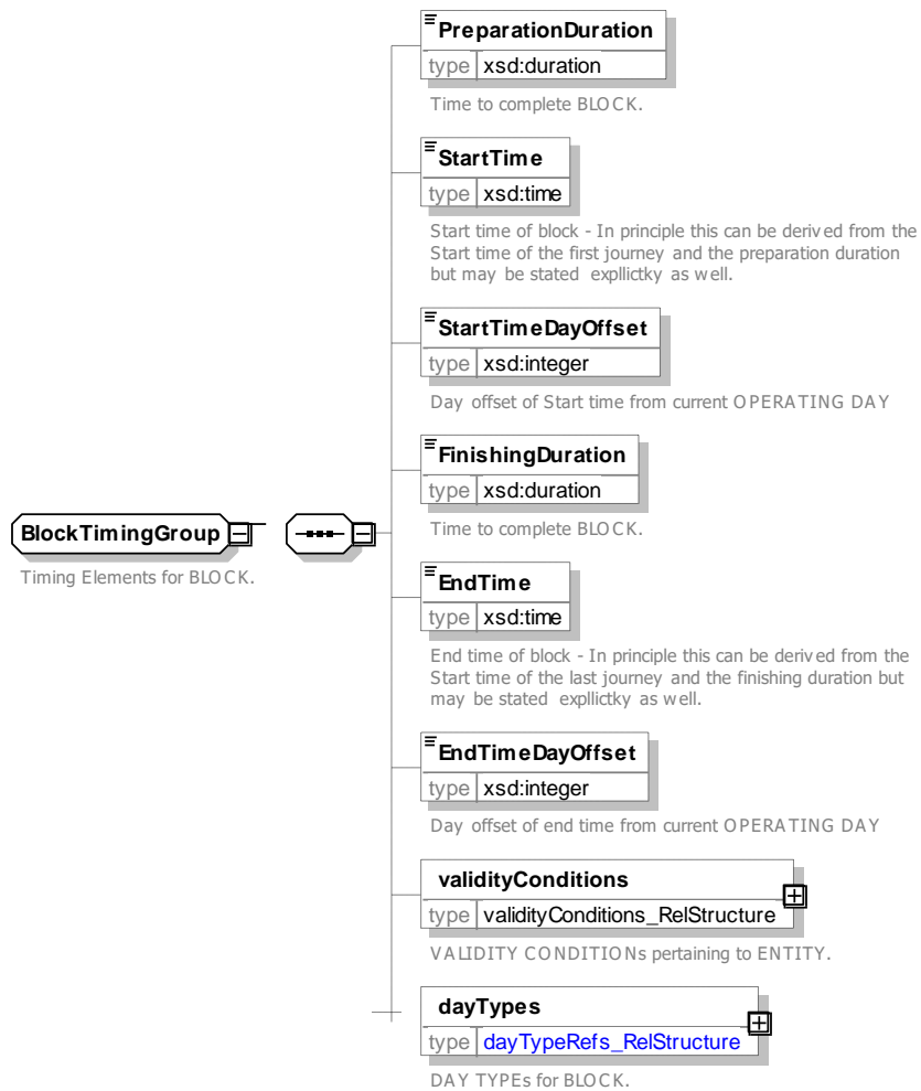
Figure 175 — BlockTimingGroup — XSD
