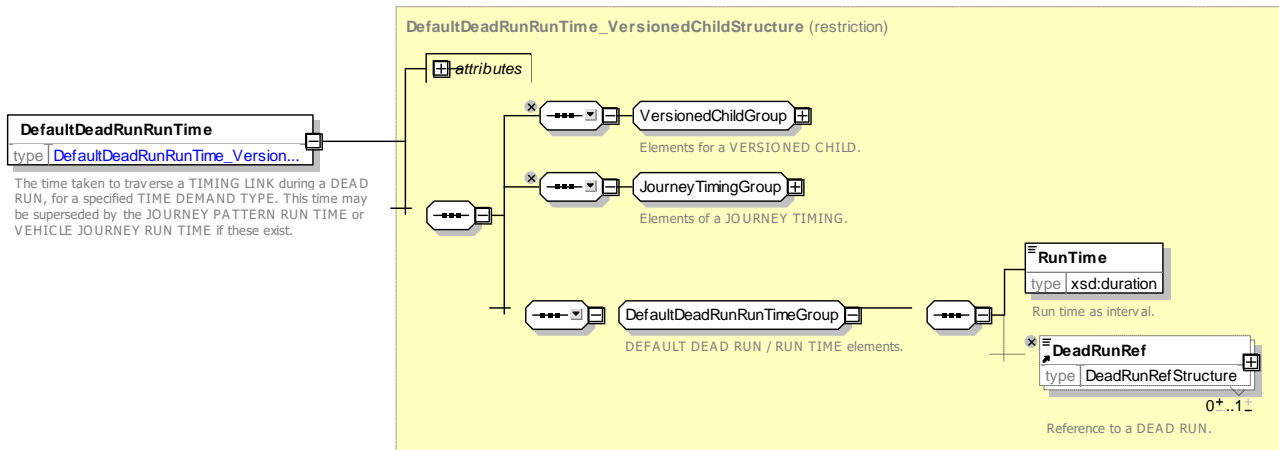
Figure 56 — DefaultDeadRunRunTimeTime — XSD
