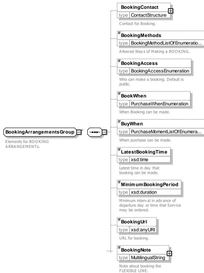
Figure 46 — BookingArrangementsGroup — XSD
