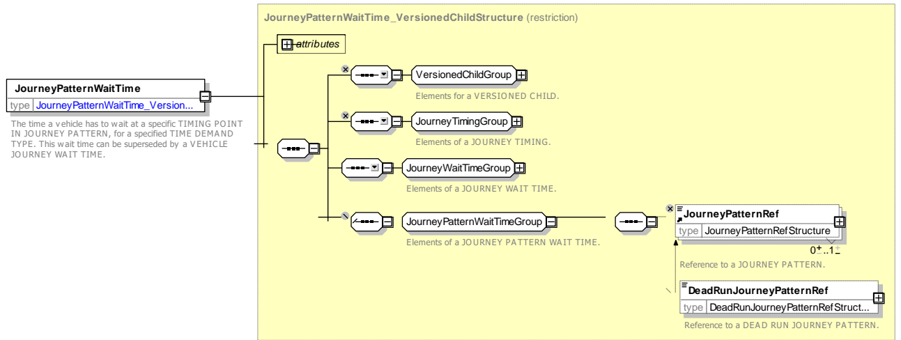
Figure 72 — JourneyPatternWaitTime — XSD
