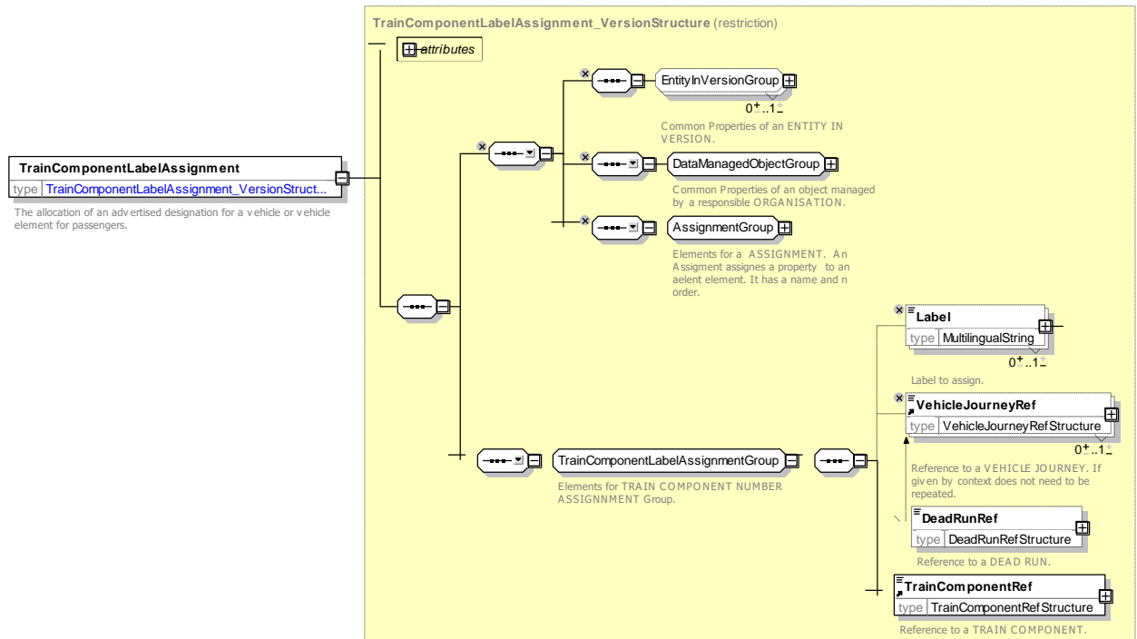
Figure 35 — TrainComponentLabelAssignment — XSD
