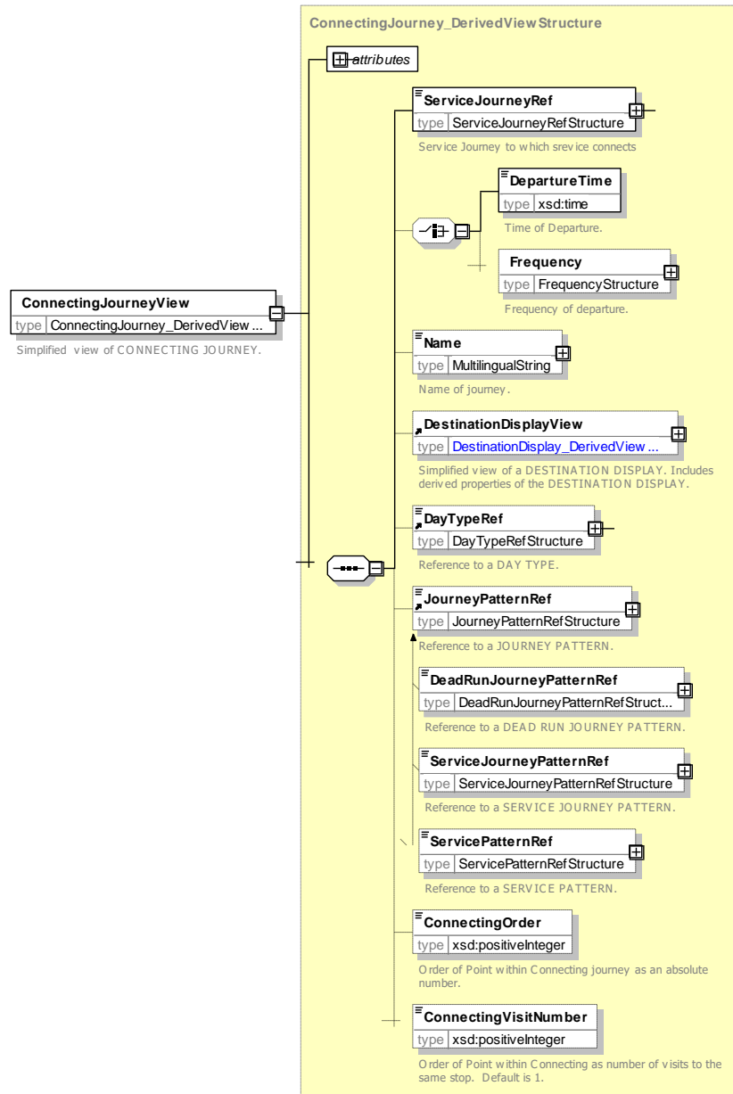
Figure 104 — ConnectingJourneyView — XSD
