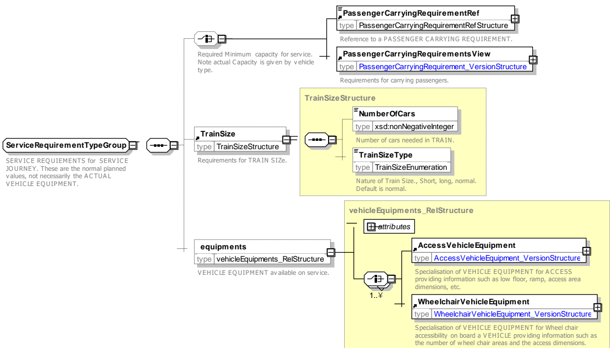
Figure 161 — ServiceRequirementTypeGroup — XSD
