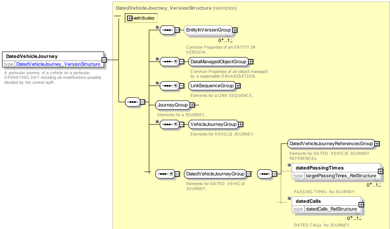
Figure 143 — DatedVehicleJourney — XSD
