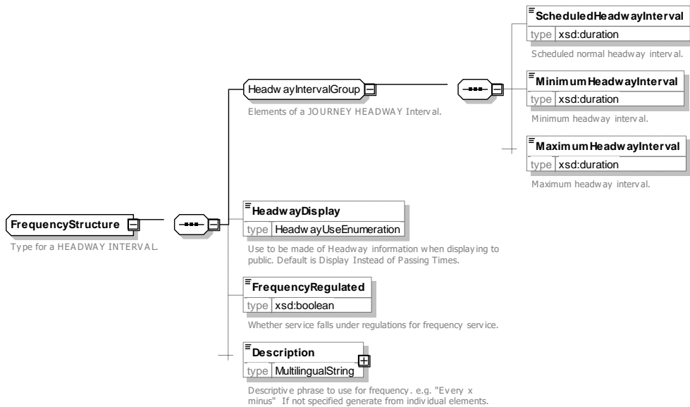
Figure 91 — JourneyFrequency — XSD
