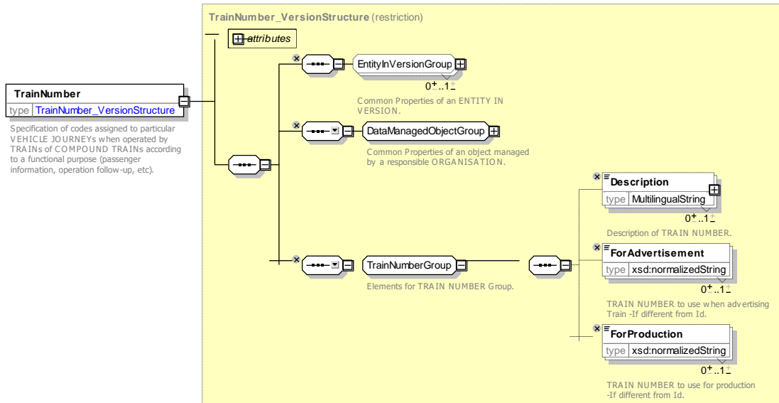
Figure 25 — TrainNumber — XSD
