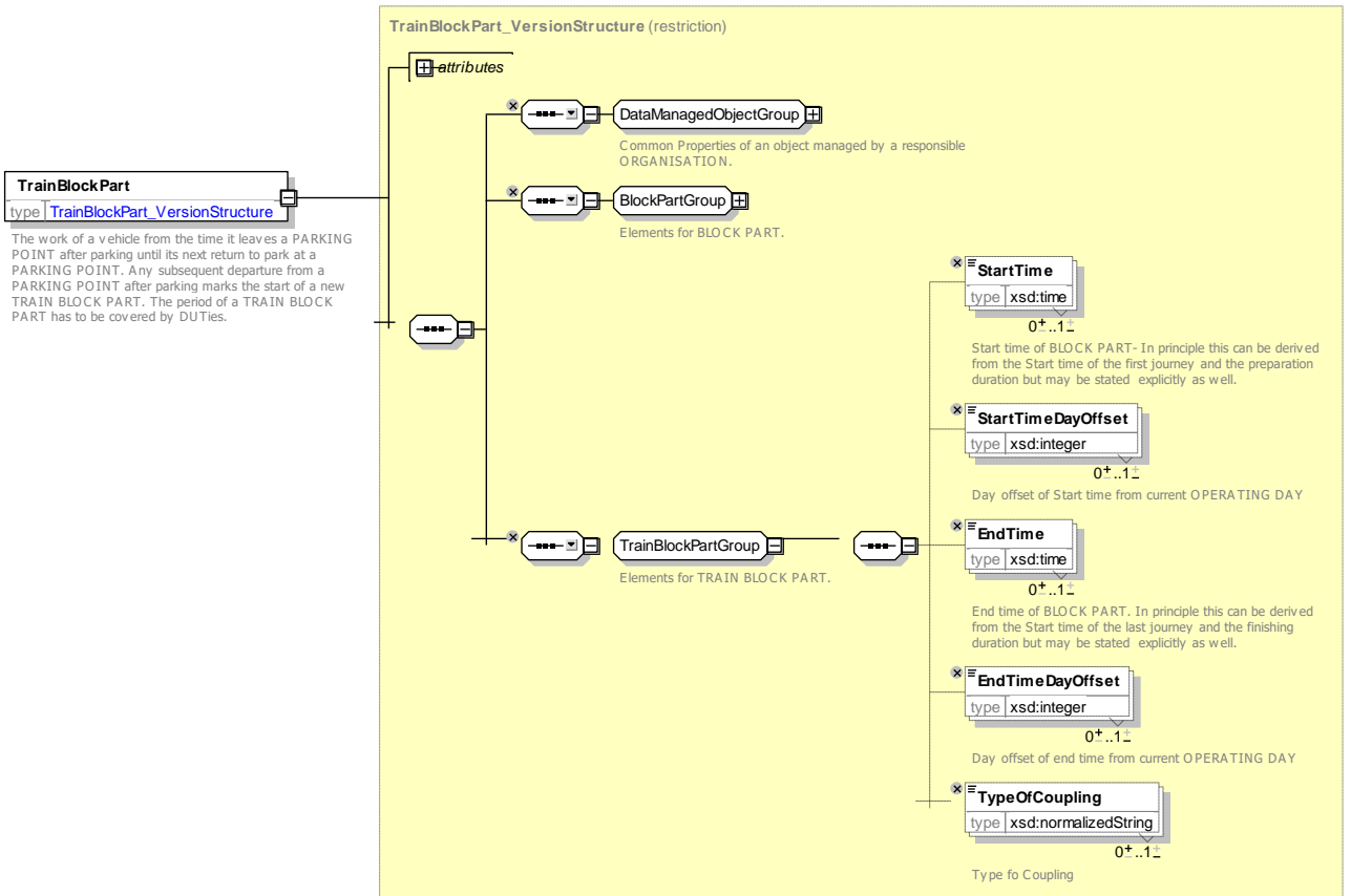
Figure 187 — TrainBlockPart — XSD
