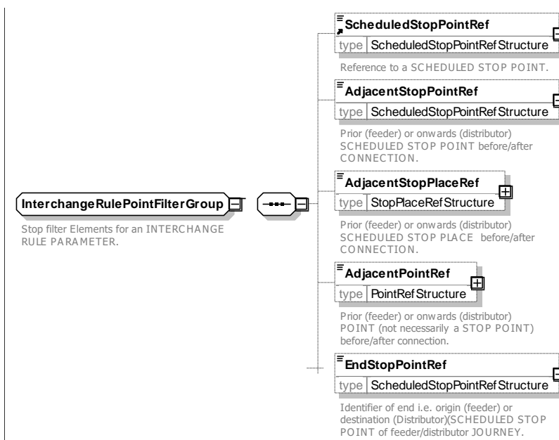
Figure 109 — InterchangeRuleParameter — XSD
