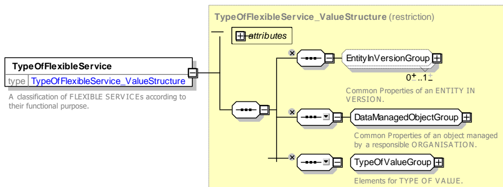
Figure 136 — TypeOfFlexibleService — XSD
