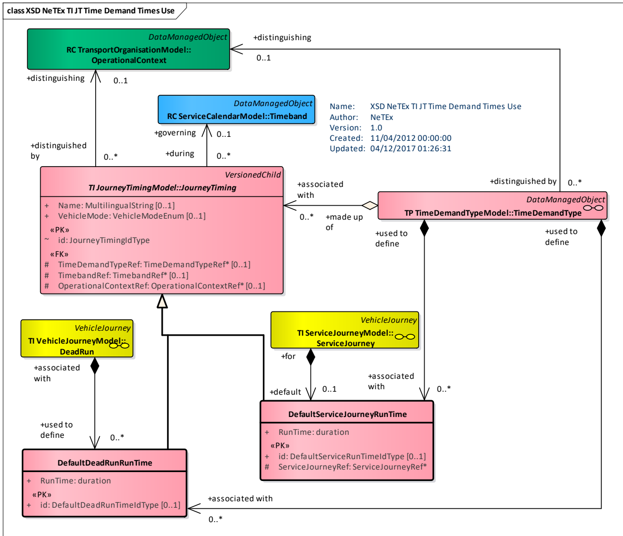
Figure 54 — Time Demand Times Use – Physical Model (UML)
