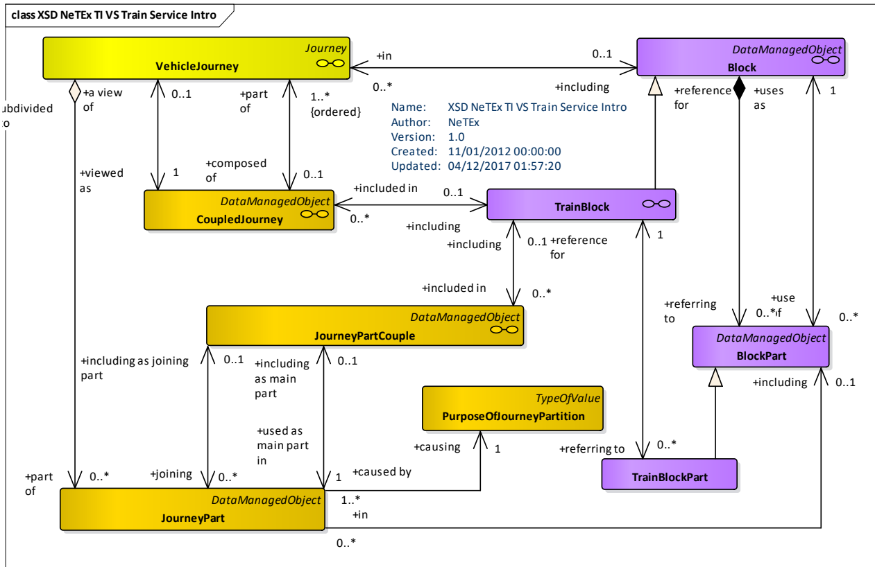
Figure 184 — Train Service Model – Conceptual MODEL (UML)
