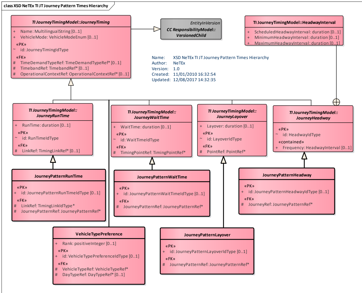
Figure 71 — Journey Pattern Times Hierarchy – Physical Model (UML)
