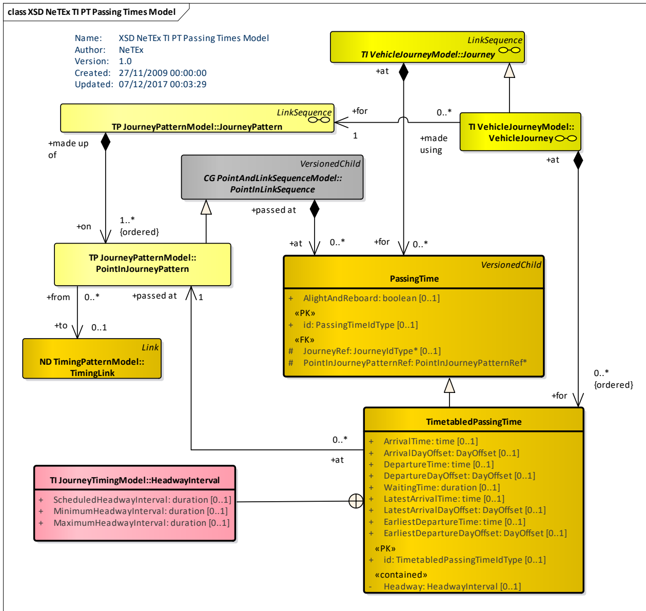
Figure 146 — Timetabled Passing Times – Physical Model (UML)
