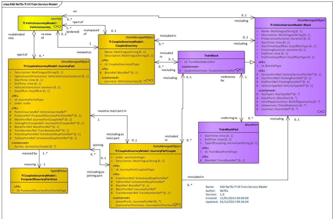
Figure 185 — Train Service Model – Physical Model (UML)
