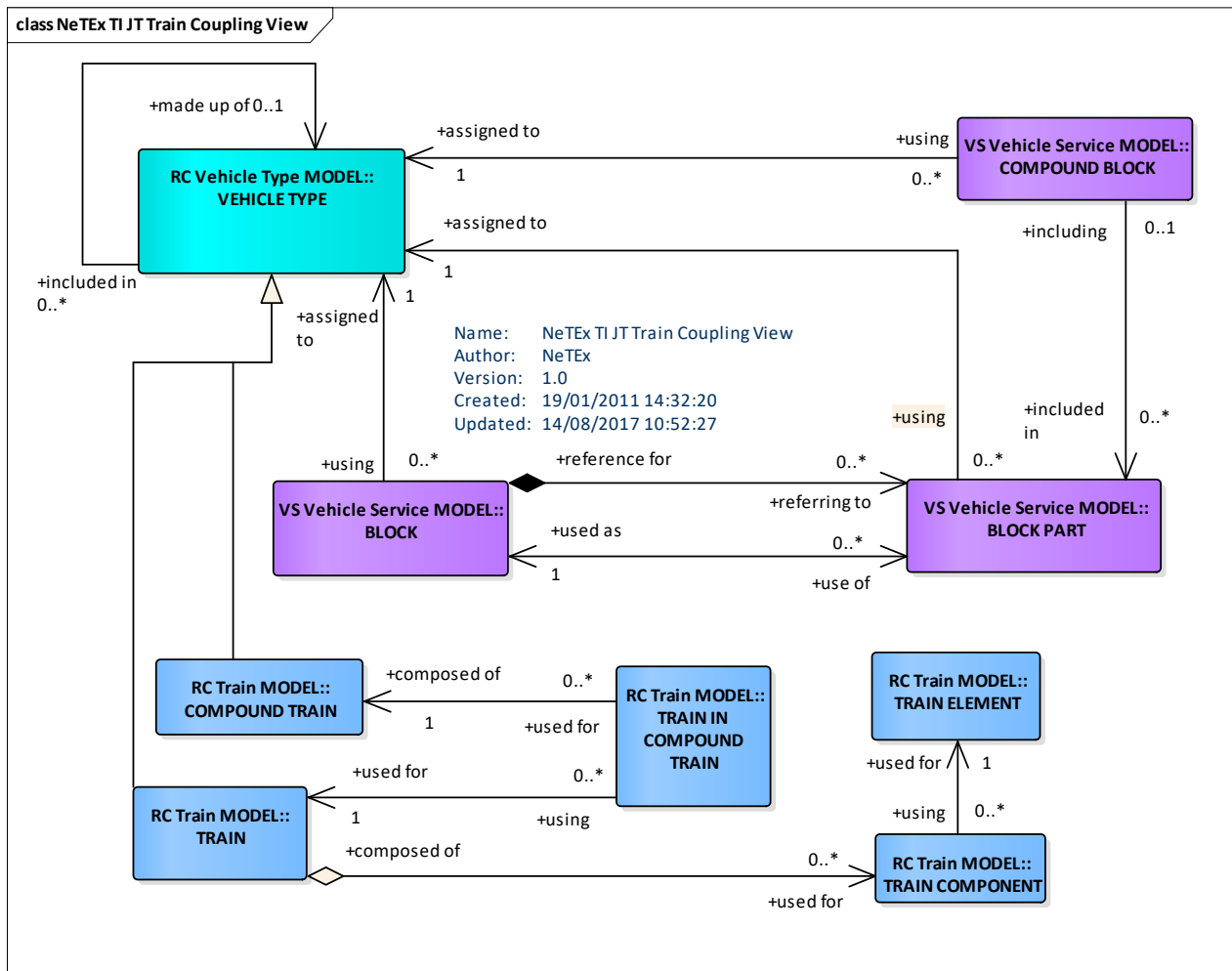
Figure 112 — Train Coupling – Conceptual MODEL (UML)
