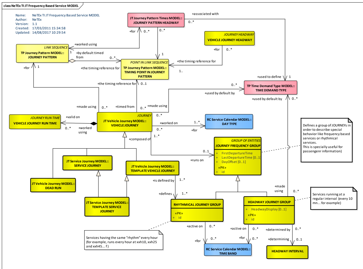
Figure 78 — Frequency Based Service – Conceptual MODEL (UML)
