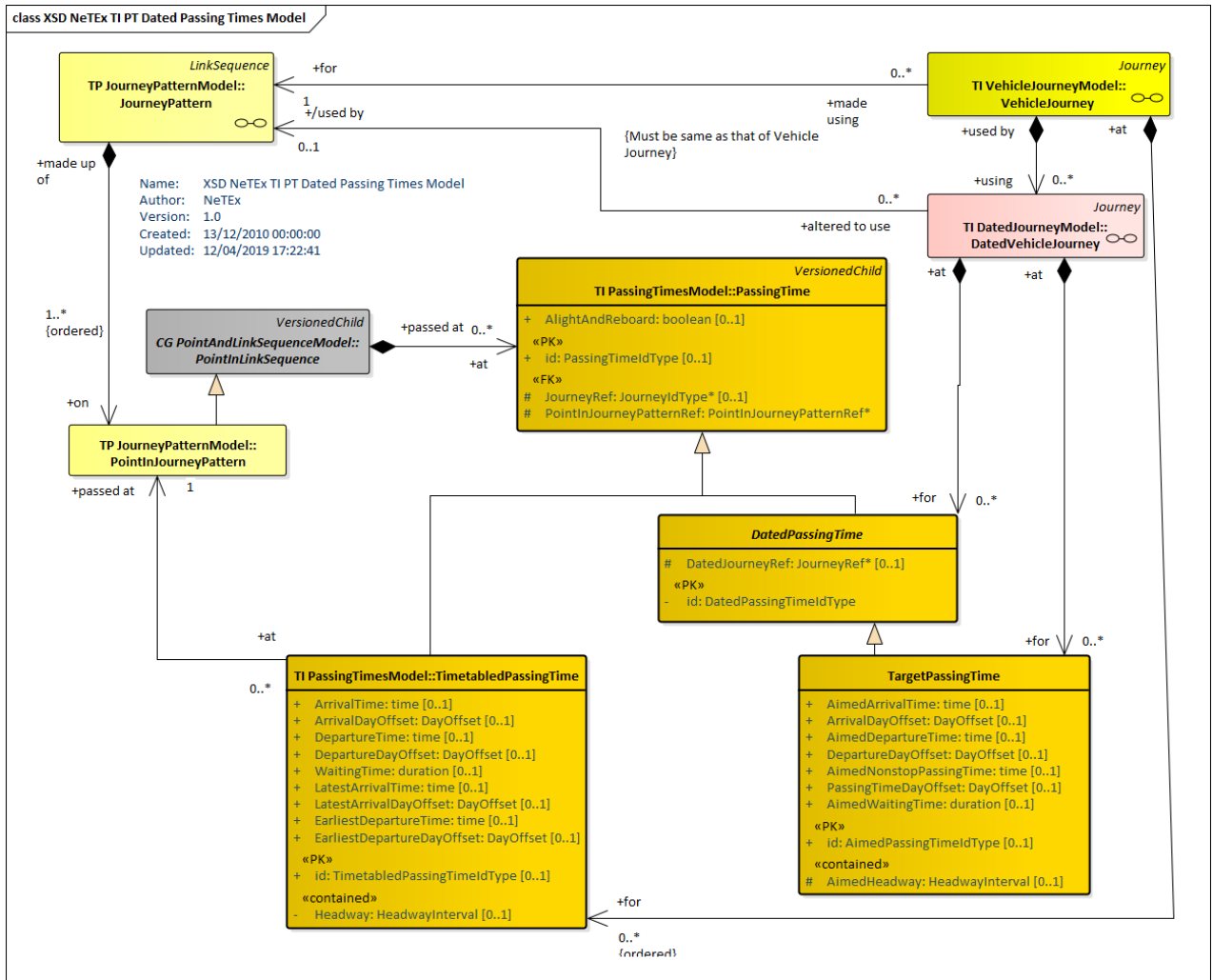
Figure 147 — Dated Passing Times – Physical Model (UML)
