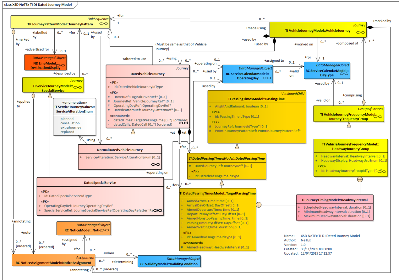
Figure 142 — Dated Journey – Physical Model (UML)
