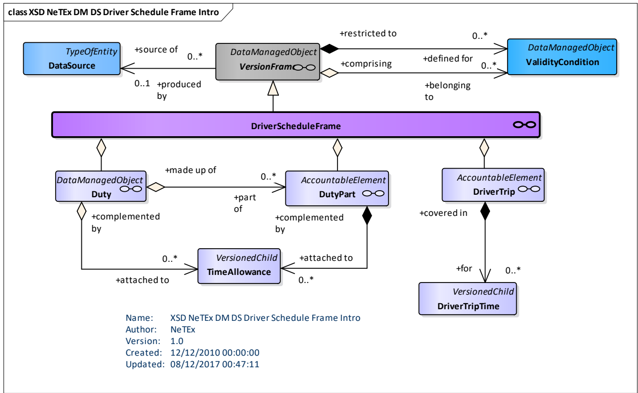
Figure 198 — Driver Schedule Frame Contents – Physical Model (UML)
