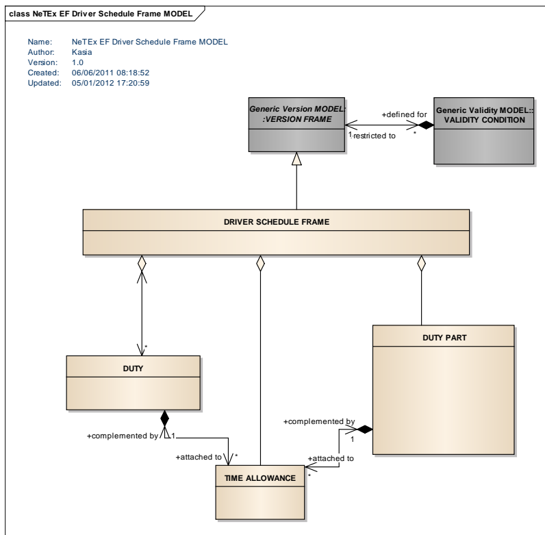
Figure 197 — Driver Schedule Frame – Conceptual MODEL (UML)
