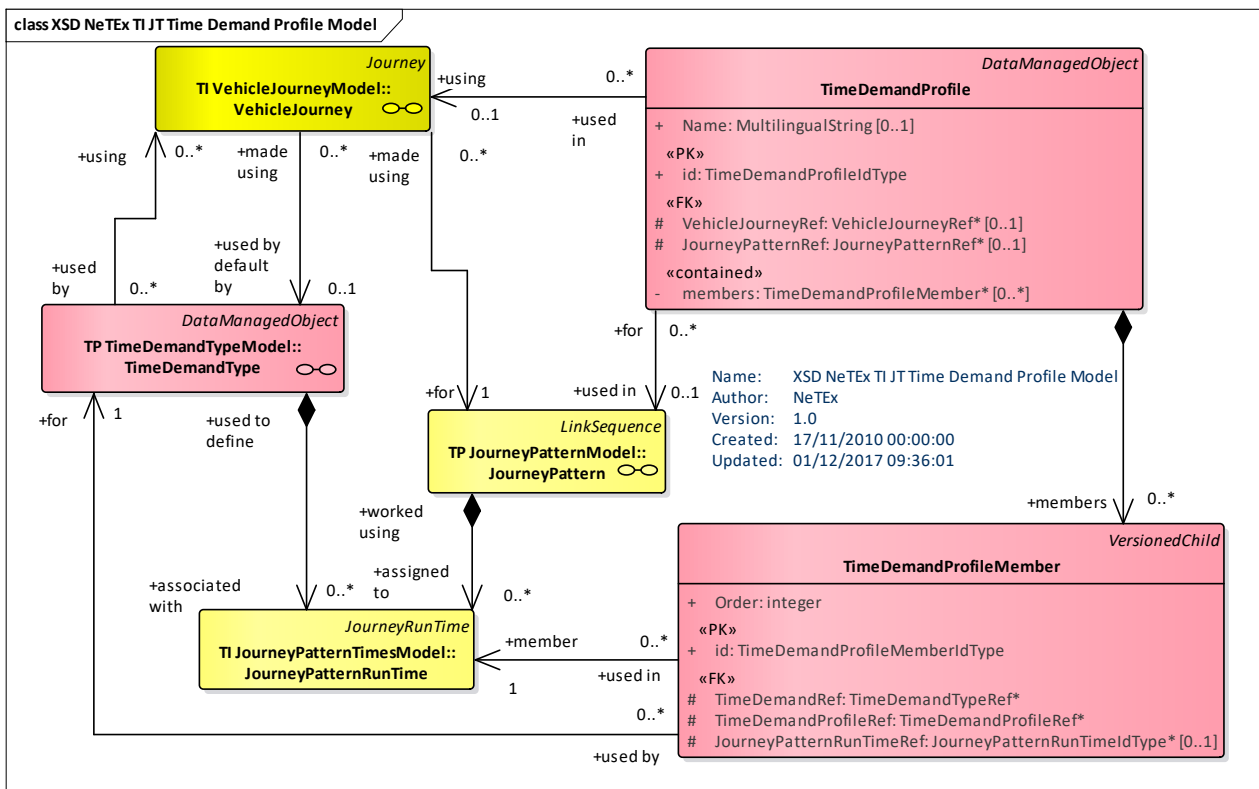
Figure 57 — Time Demand Profile – Physical Model (UML)
