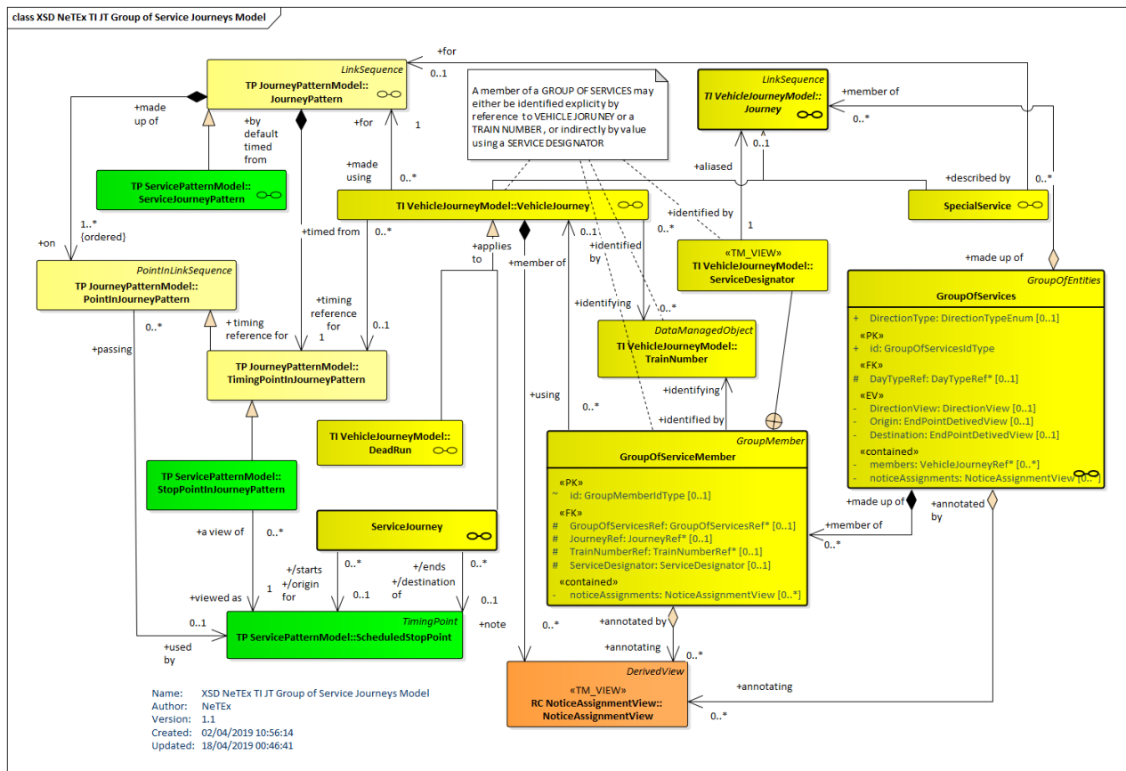
Figure 39 — Group of Services – Physical Model (UML)
