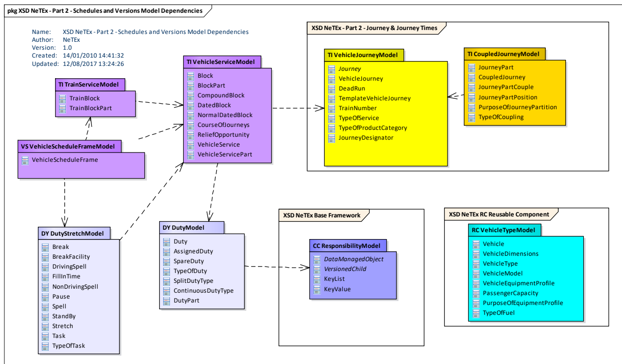
Figure 167 — Vehicle Schedules – Model Dependencies
