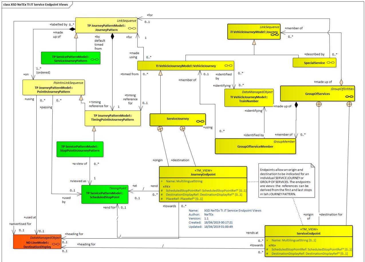
Figure 40 — Service Endpoints – Physical Model (UML)
