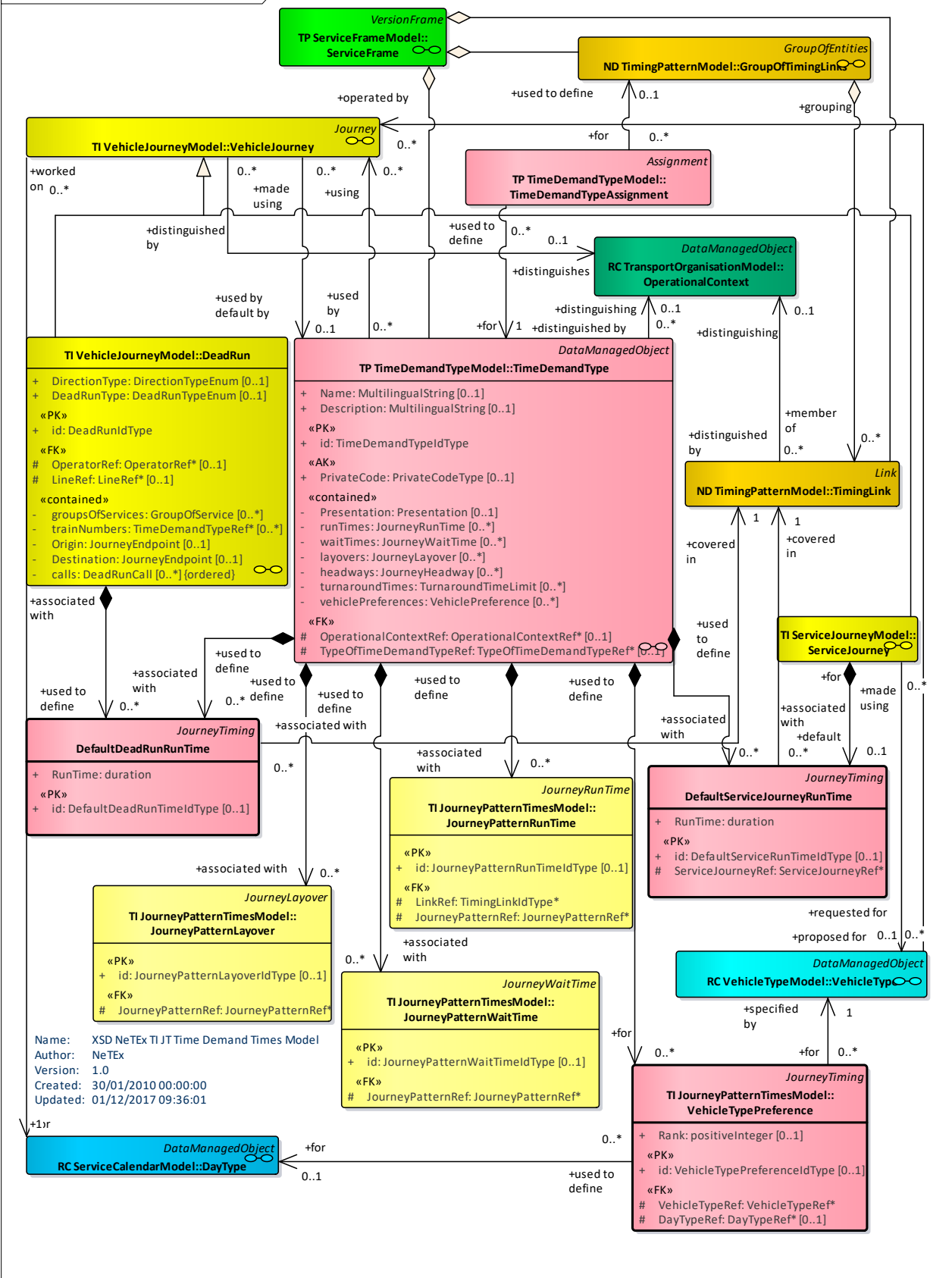
Figure 53 — Time Demand Times – Physical Model (UML)
