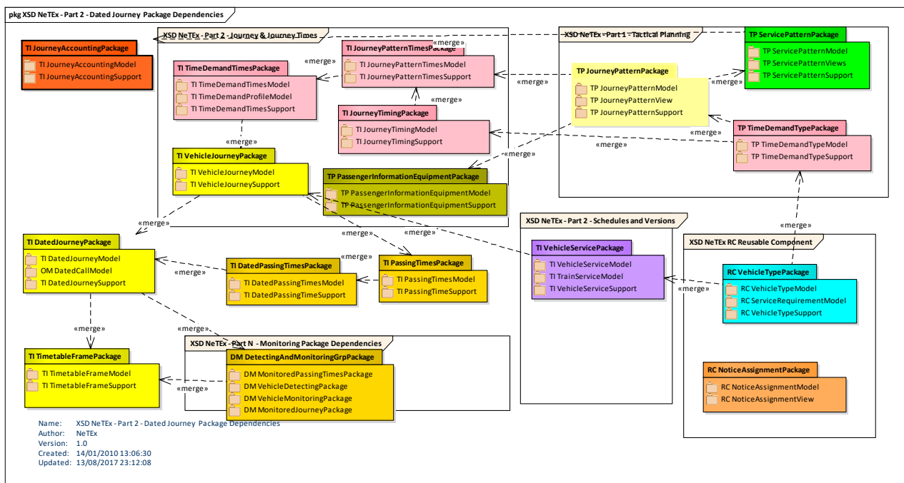
Figure 140 — Dated Journey Package Dependencies
