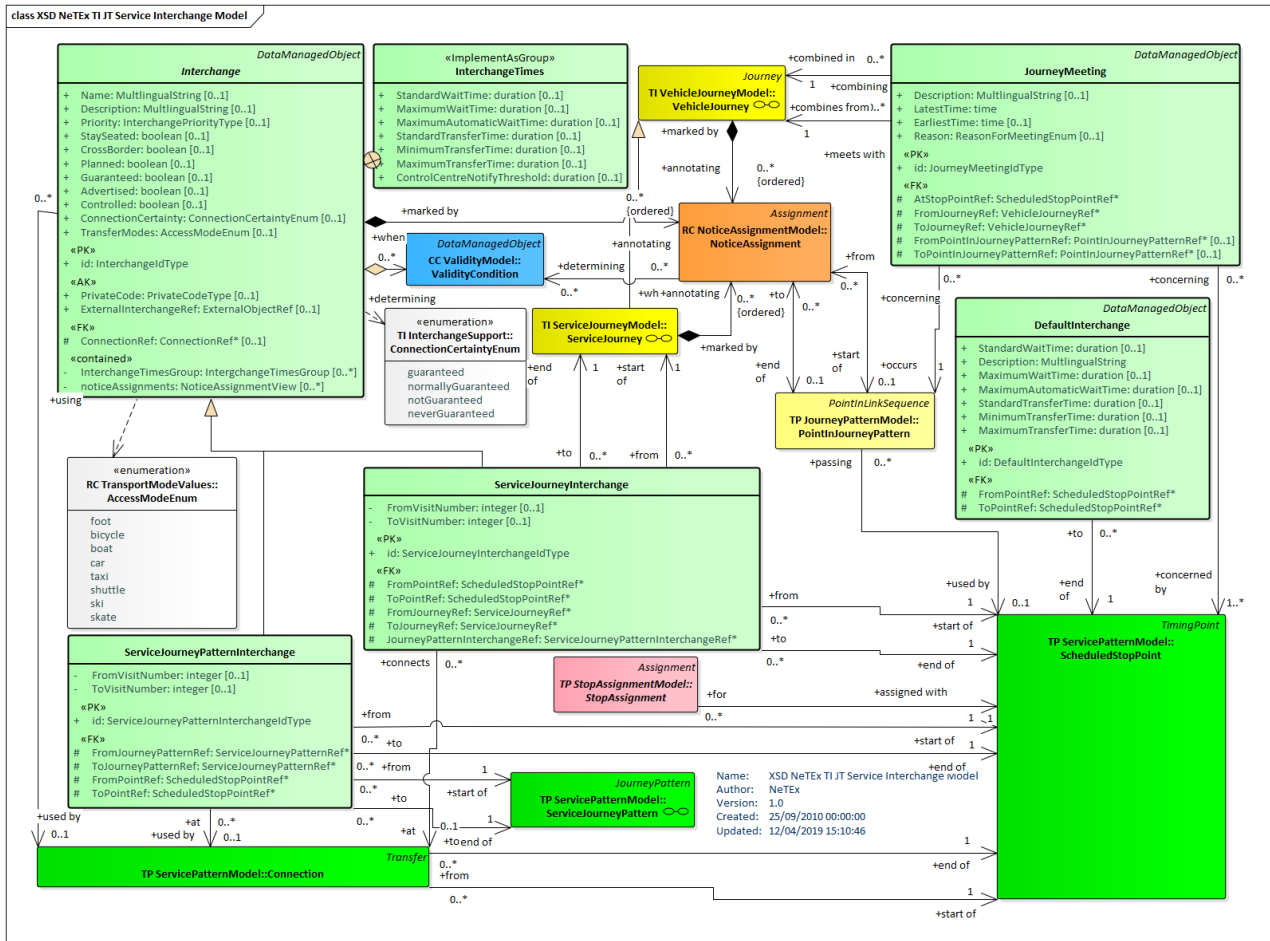
Figure 93 — Service Interchange – Physical Model (UML)
