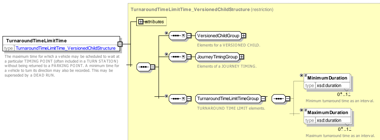
Figure 68 — TurnaroundTimeLimitTime — XSD
