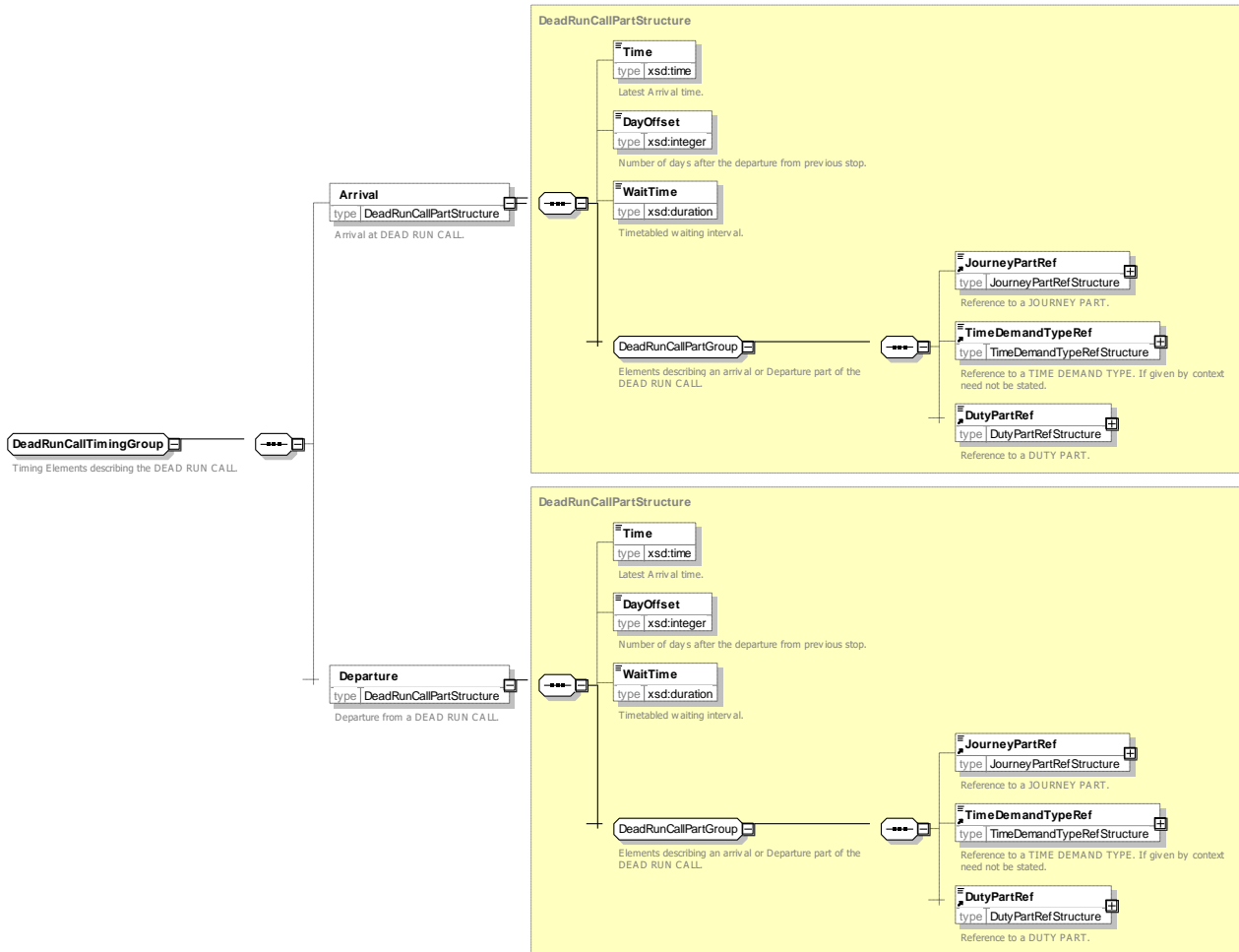
Figure 163 — DeadRunTimingGroup — XSD
