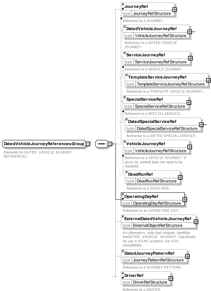
Figure 144 — DatedVehicleJourneyReferencesGroup — XSD
