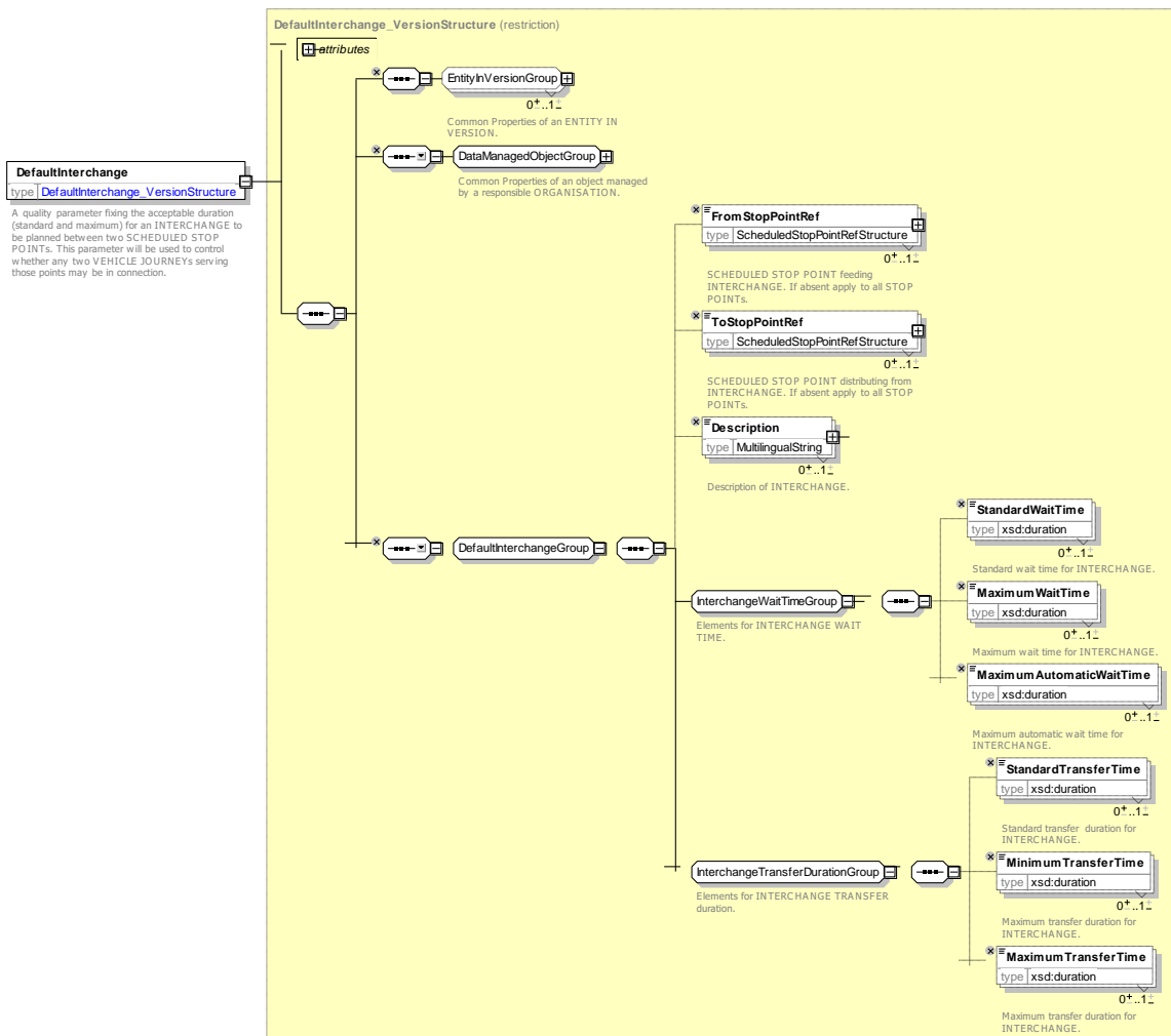
Figure 94 — DefaultInterchange — XSD
