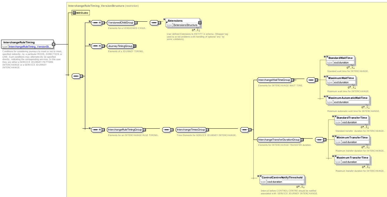
Figure 111 — InterchangeRuleTiming — XSD
