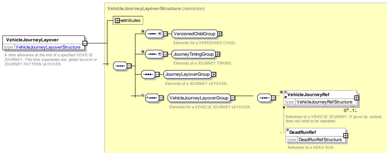
Figure 83 — VehicleJourneyLayover — XSD
