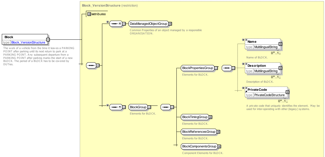
Figure 174 — Block — XSD
