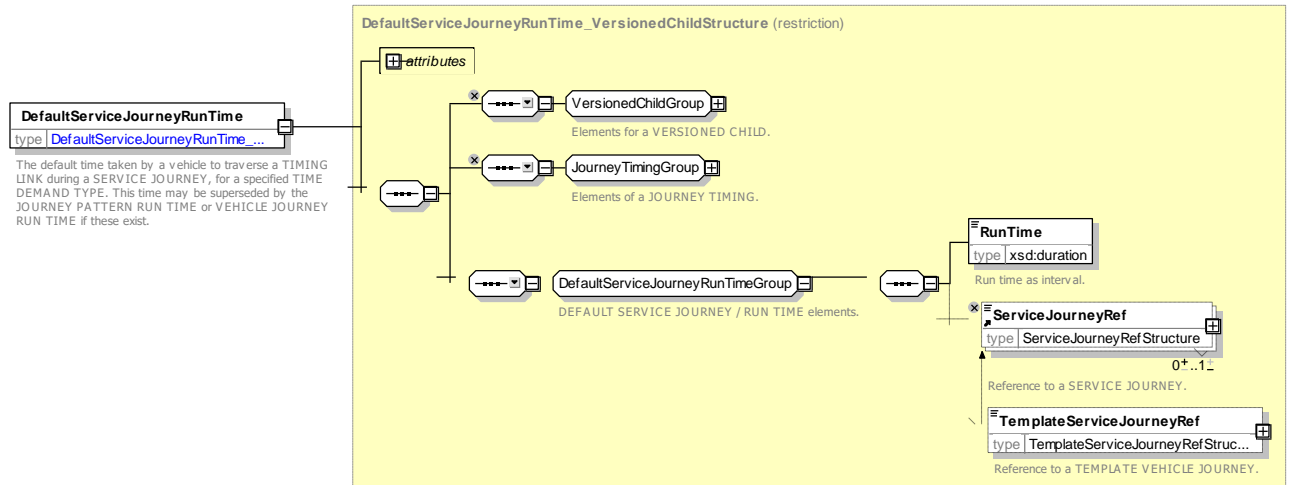
Figure 55 — DefaultServiceJourneyRunTime — XSD
