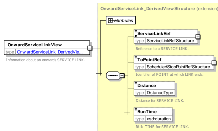
Figure 157 — OnwardServiceLinkView — XSD
