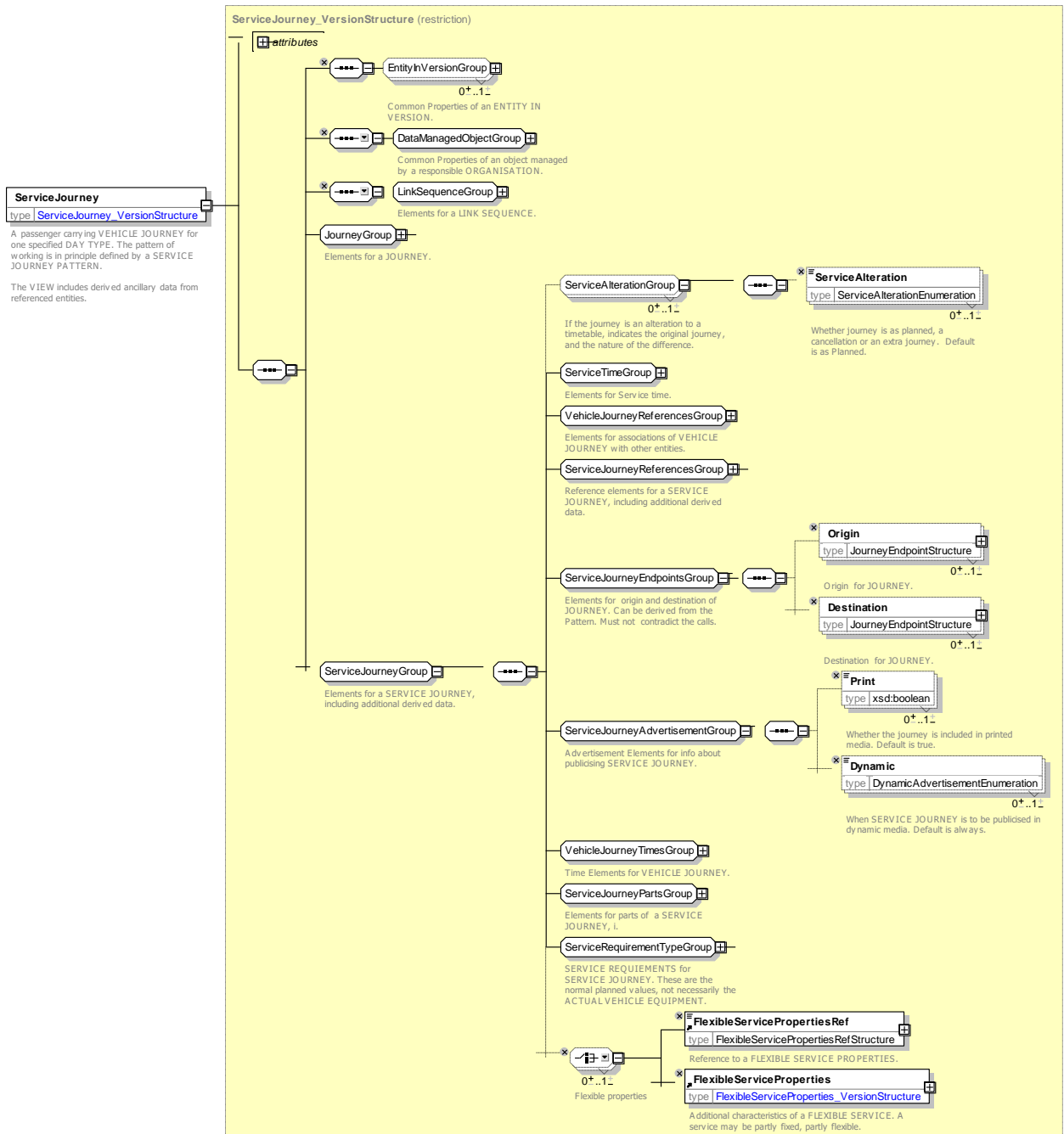
Figure 41 — ServiceJourney — XSD
