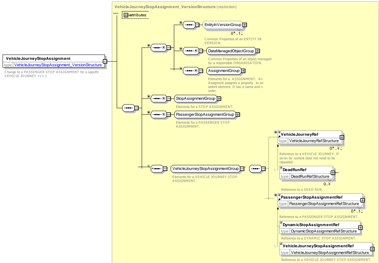
Figure 33 — VehicleJourneyStopAssignment — XSD
