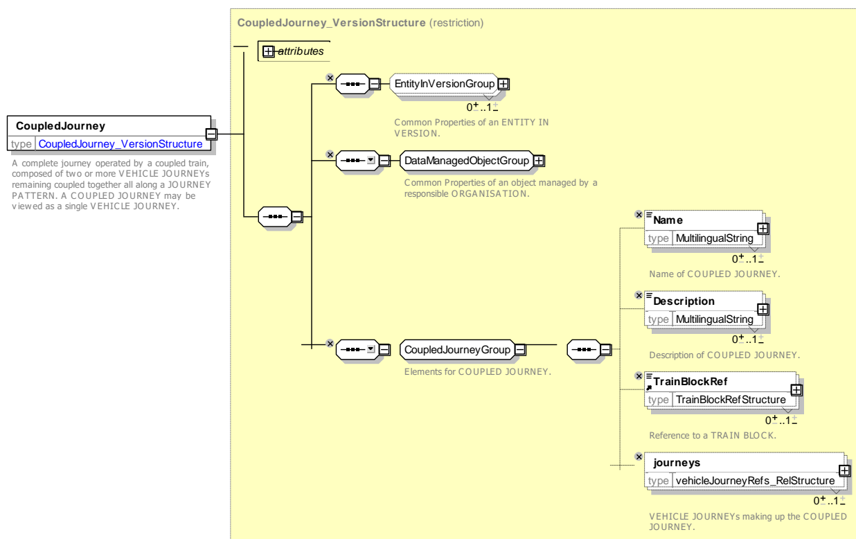
Figure 126 — CoupledJourney — XSD
