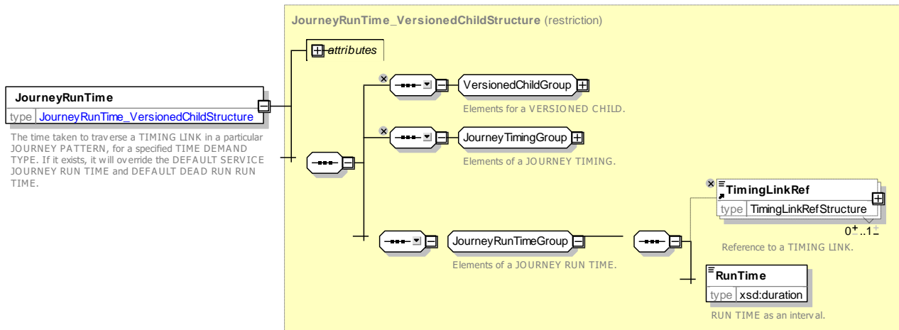
Figure 64 — JourneyRunTime — XSD
