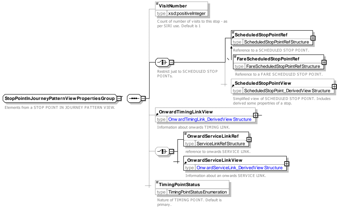
Figure 154 — StopPointInJourneyPatternViewPropertiesGroup — XSD
