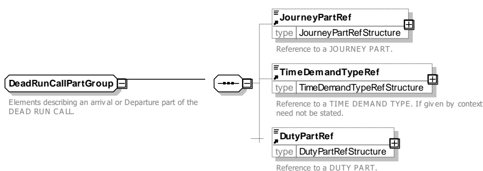
Figure 164 — DeadRunCallPart — XSD
