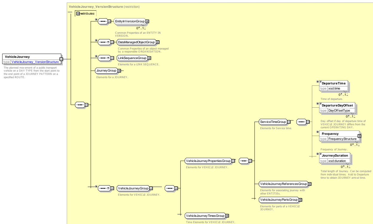
Figure 17 — VehicleJourney — XSD
