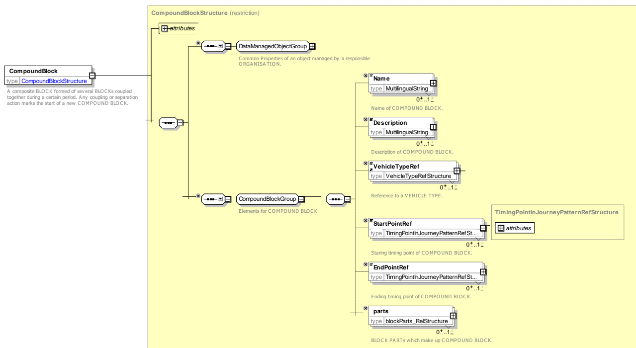
Figure 179 — CompoundBlock — XSD
