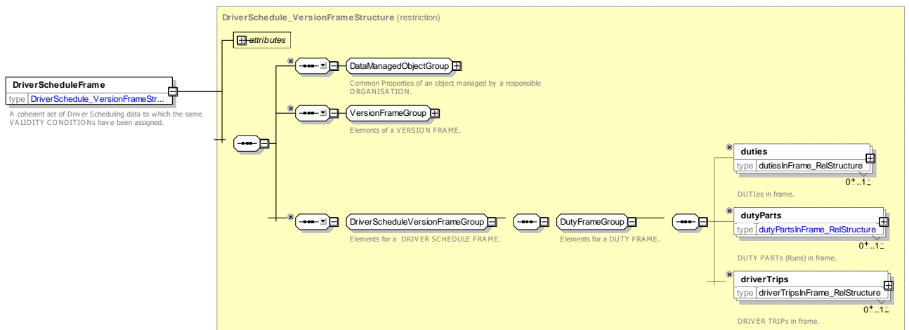
Figure 200 — DriverScheduleFrame — XSD
