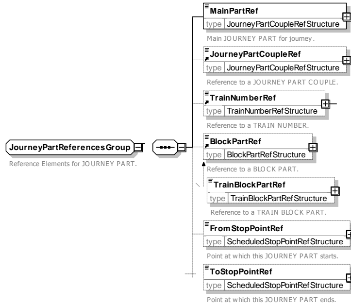
Figure 125 — JourneyPartReferencesGroup — XSD
