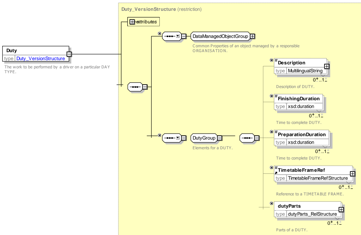
Figure 203 — Duty — XSD
