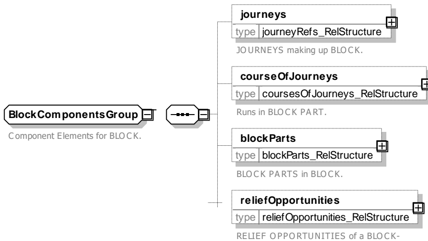
Figure 177 — BlockComponentsGroup — XSD
