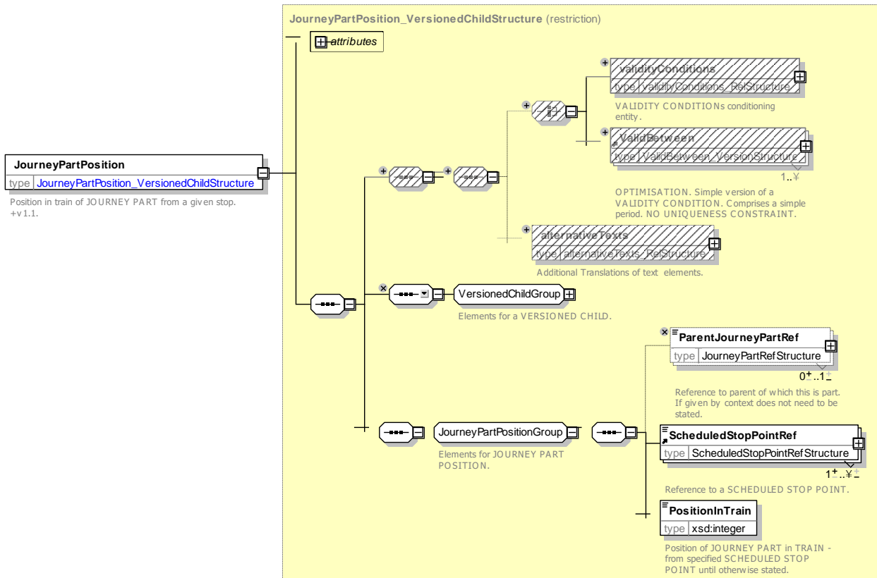
Figure 129 — JourneyPartPosition — XSD
