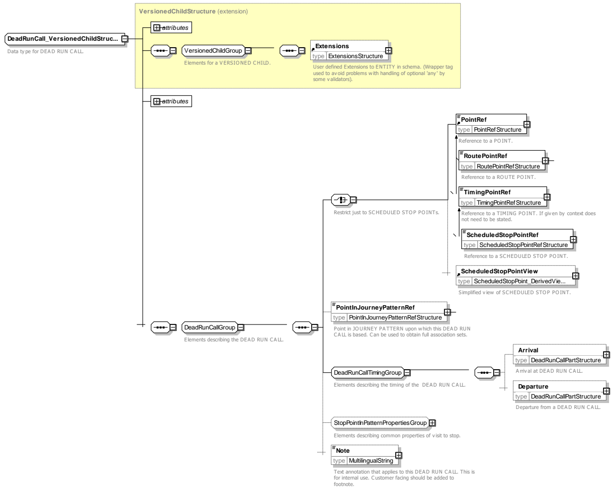
Figure 162 — DeadRunCall — XSD
