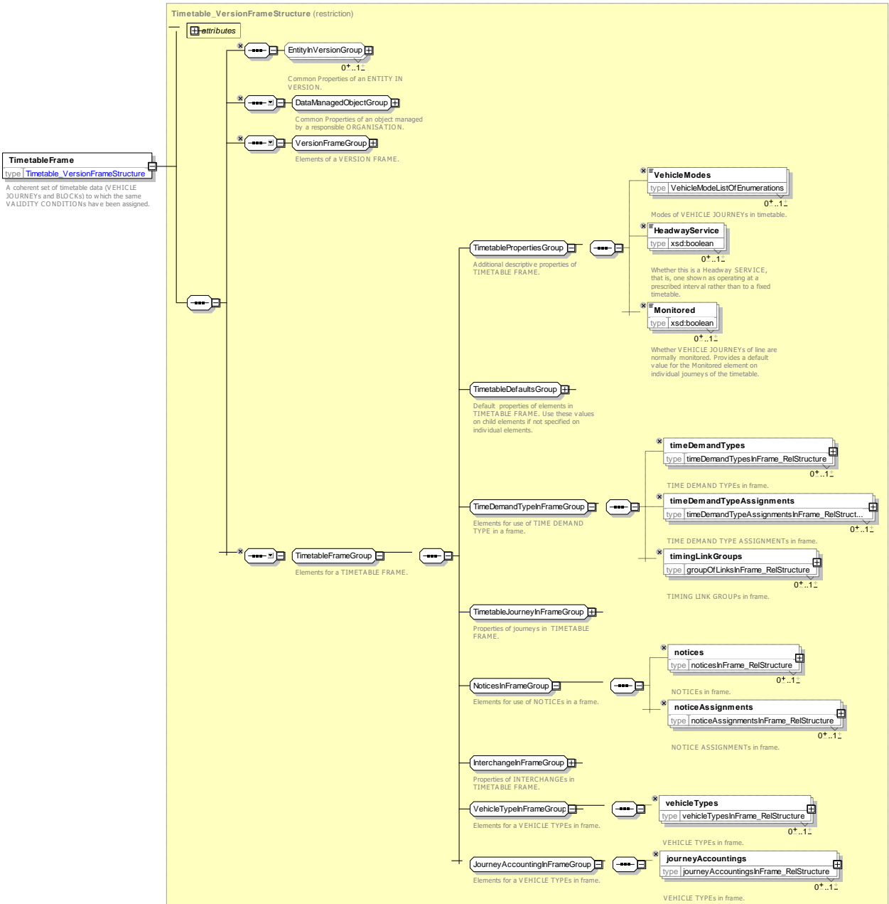
Figure 7 — TimetableFrame — XSD
