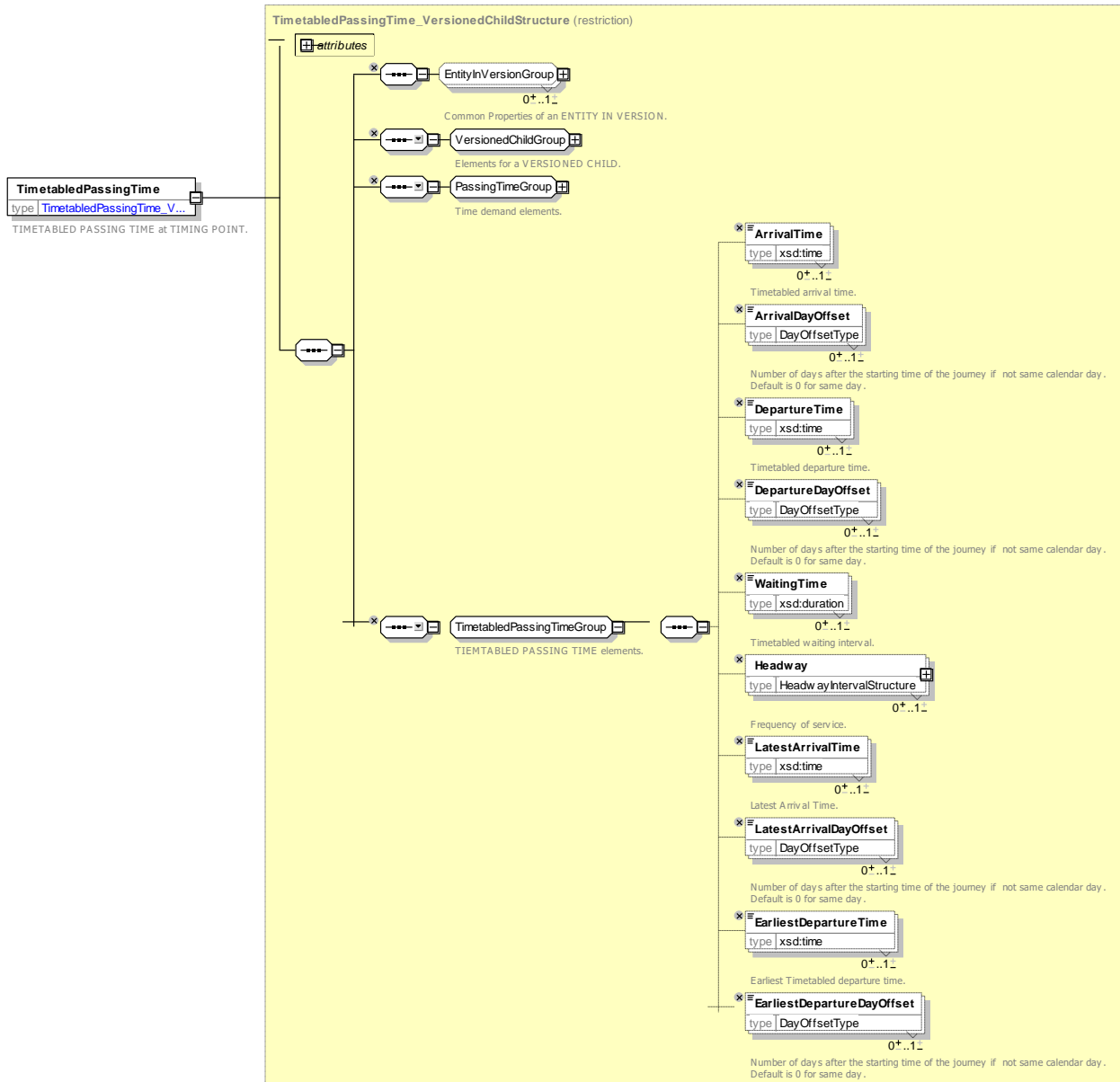
Figure 149 — TimetabledPassingTime — XSD
