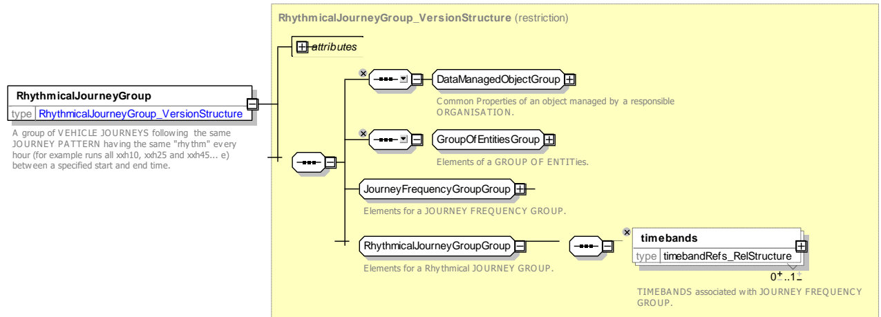
Figure 89 — RhythmicalJourneyGroup — XSD
