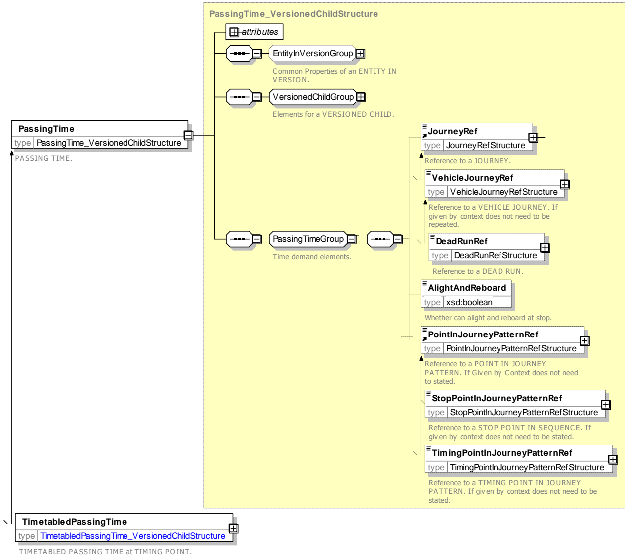
Figure 148 — PassingTime — XSD
