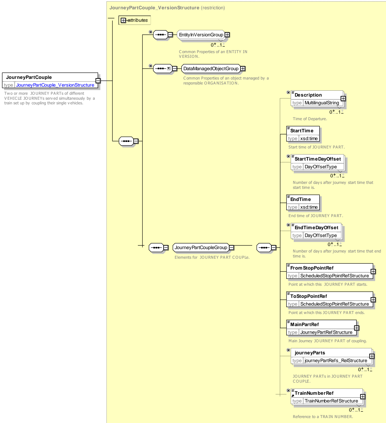
Figure 127 — JourneyPartCouple — XSD
