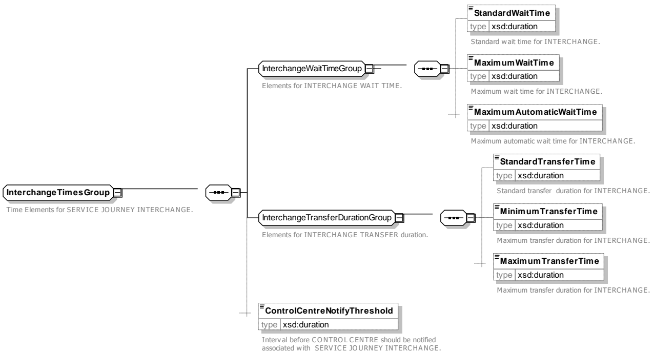
Figure 97 — InterchangeTimesGroup — XSD
