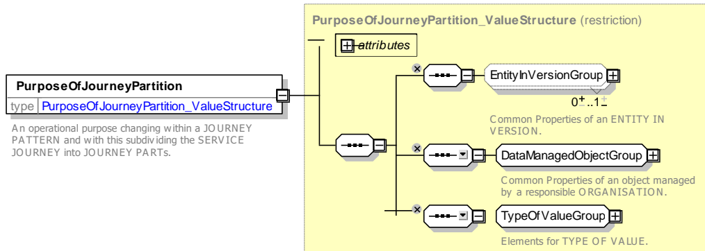
Figure 128 — PurposeOfJourneyPartition — XSD
