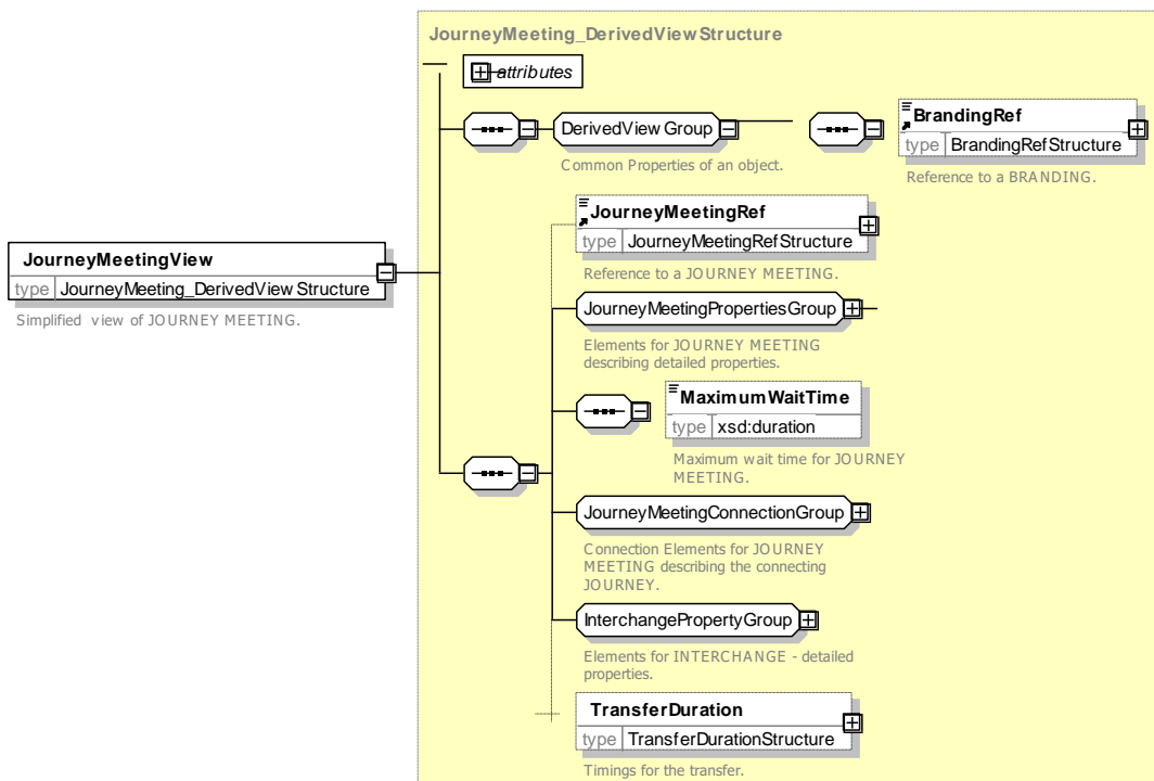
Figure 103 — JourneyMeetingView — XSD
