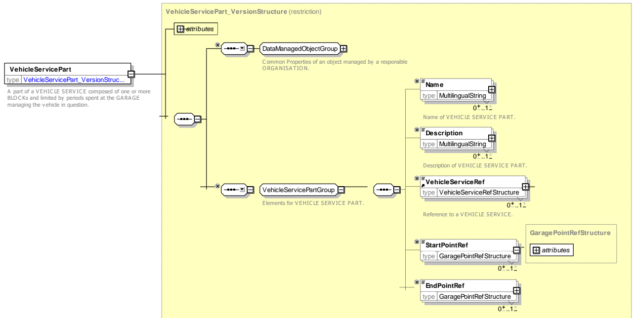
Figure 183 — VehicleServicePart — XSD
