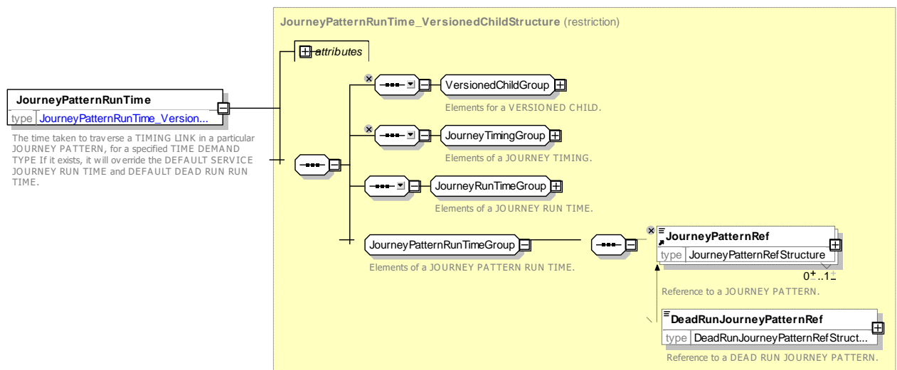
Figure 73 — JourneyPatternRunTime — XSD
