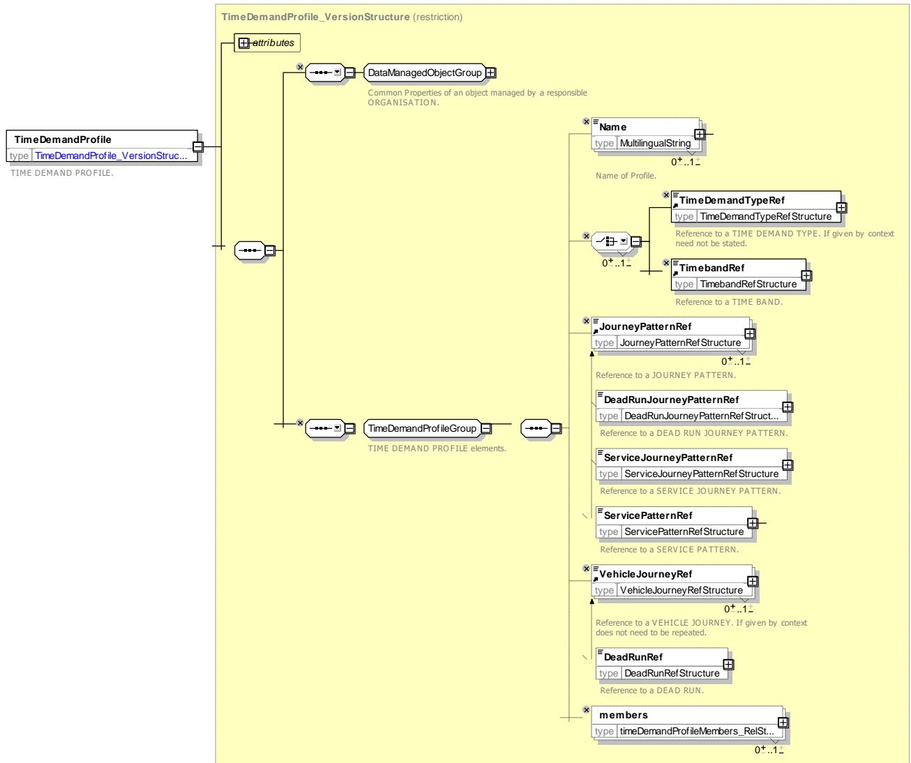
Figure 58 — TimeDemandProfile — XSD
