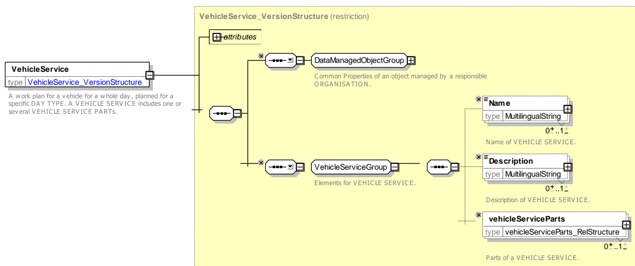
Figure 182 — VehicleService — XSD
