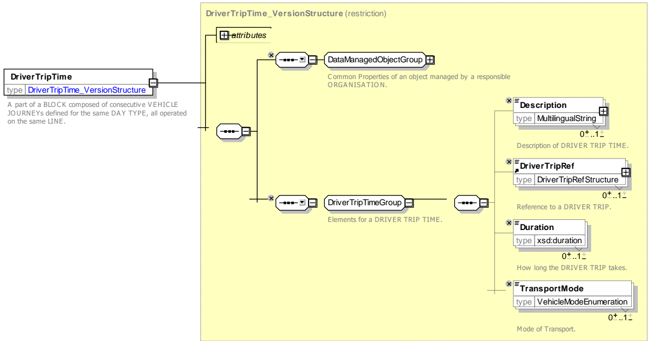
Figure 207 — DriverTripTime — XSD
