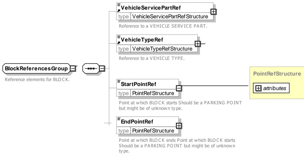
Figure 176 — BlockReferencesGroup — XSD
