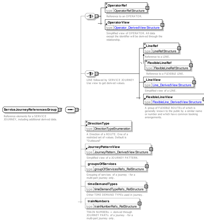
Figure 42 — ServiceJourneyReferencesGroup — XSD
