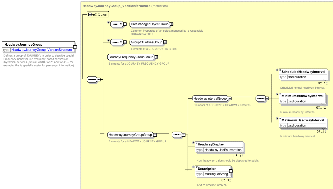
Figure 88 — HeadwayJourneyGroup — XSD
