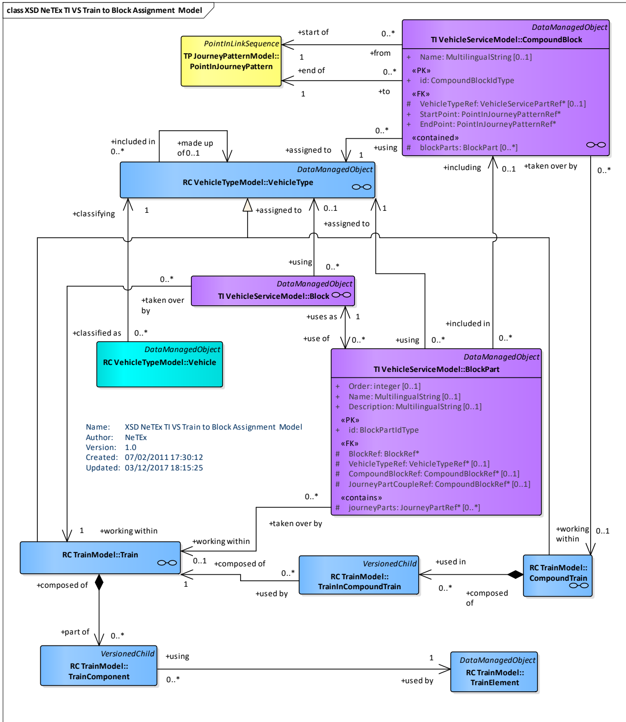
Figure 123 — Train to Block Assignment – Physical Model (UML)
