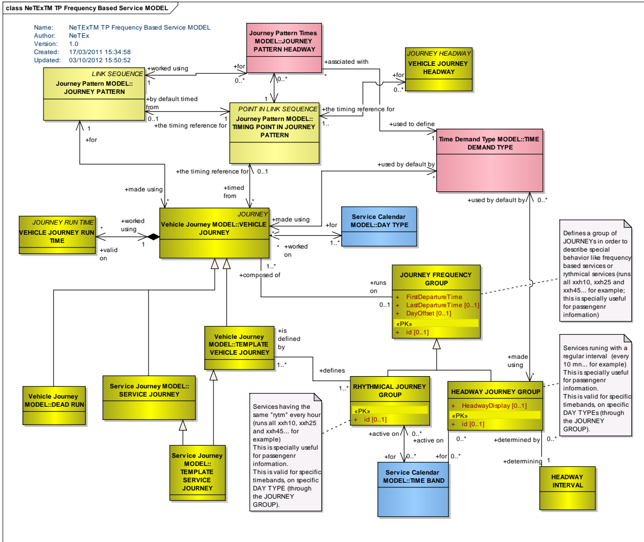
Figure 85 — Vehicle Journey Frequency – Conceptual MODEL (UML)
