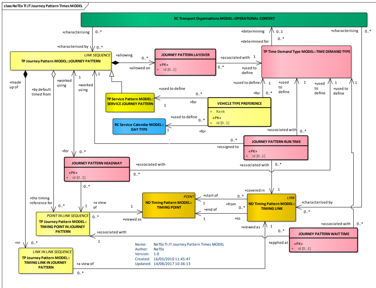
Figure 69 — Journey Pattern Times – Conceptual MODEL (UML)
