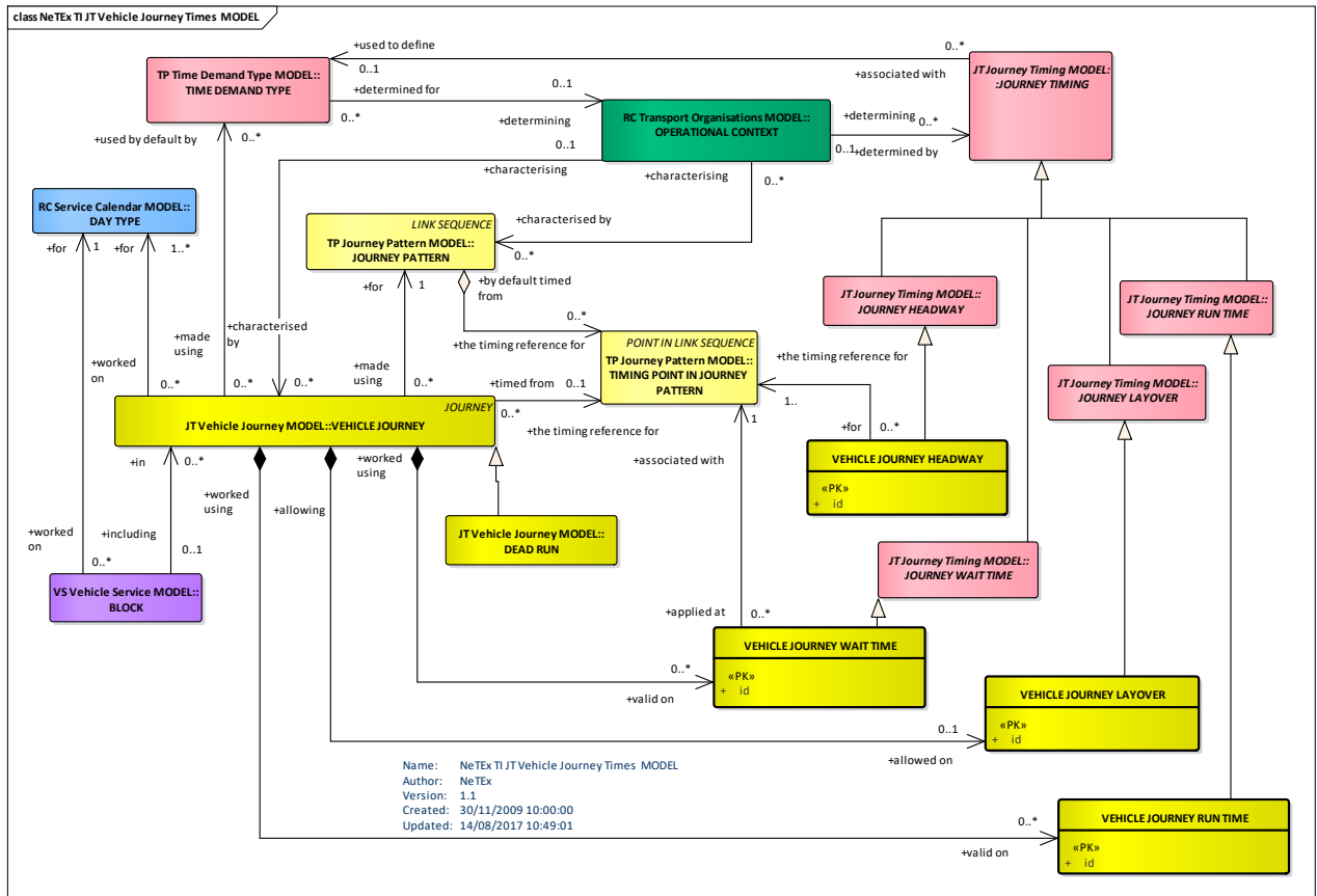
Figure 77 — Vehicle Journey Times — Conceptual MODEL (UML)
