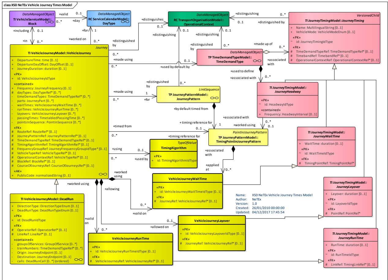
Figure 79 — Vehicle Journey Times – Physical Model (UML)
