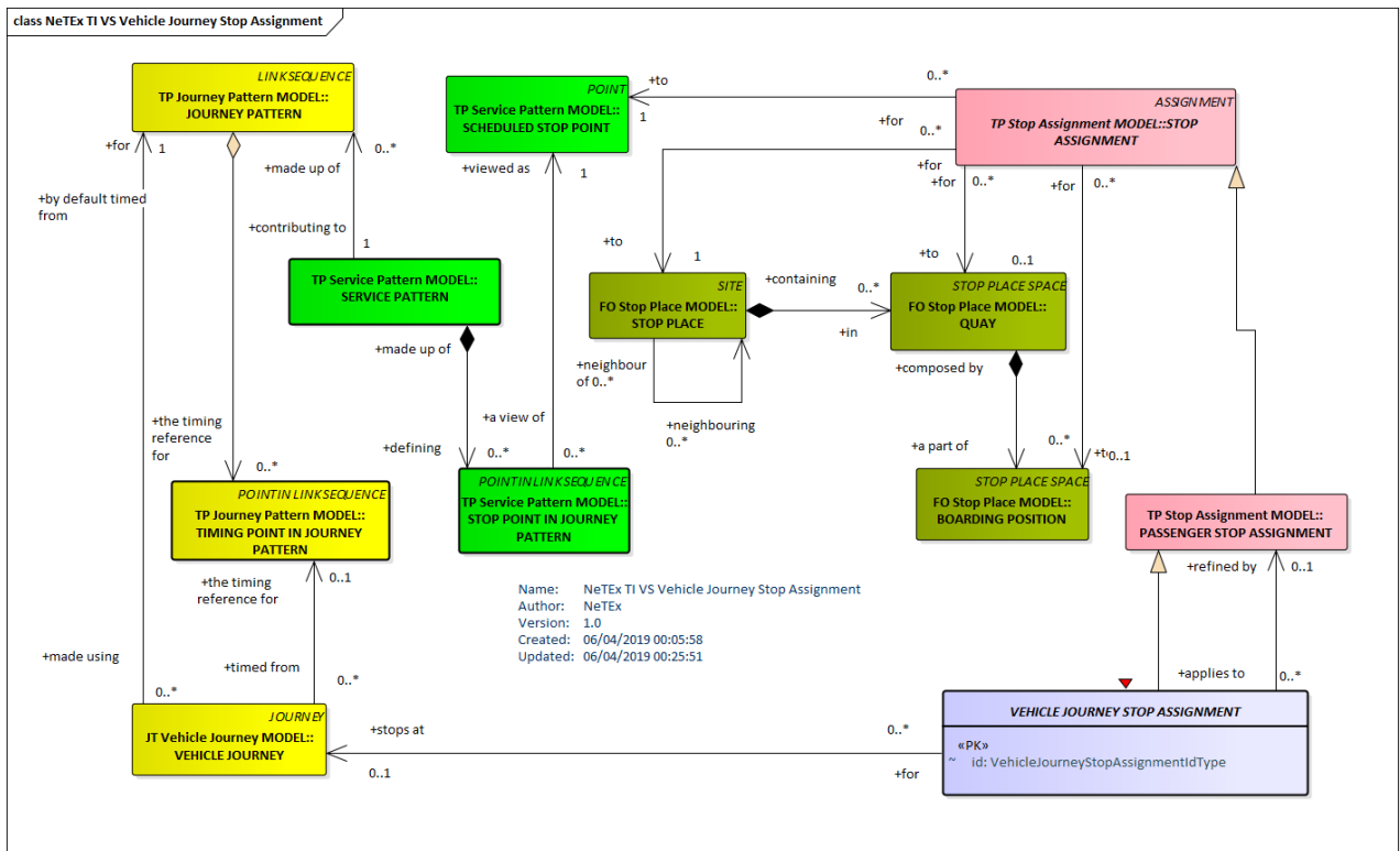
Figure 28 — Vehicle Journey Stop Assignment – Conceptual MODEL (UML)
