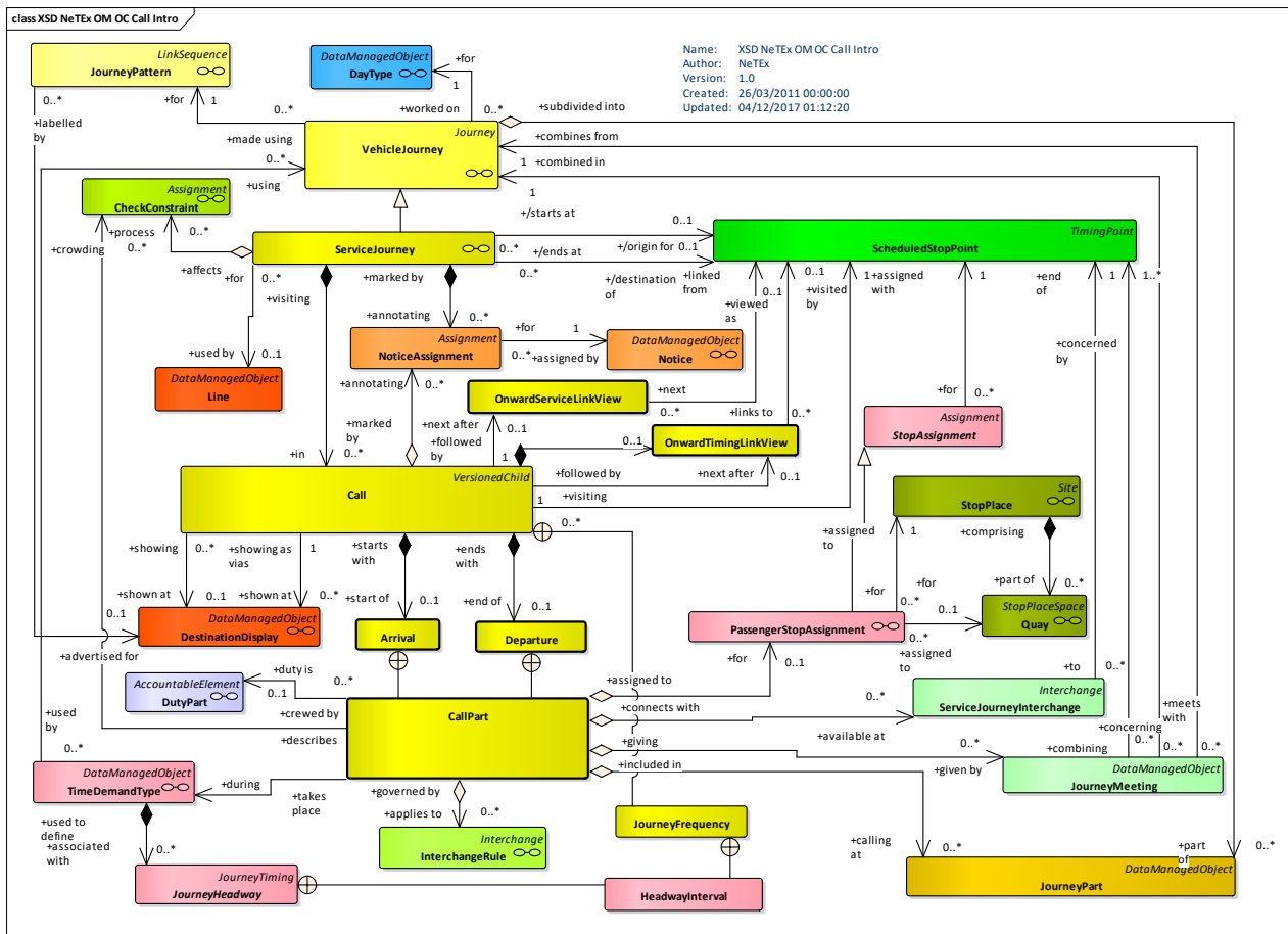
Figure 80 — Call: Overview – Physical Model (UML)
