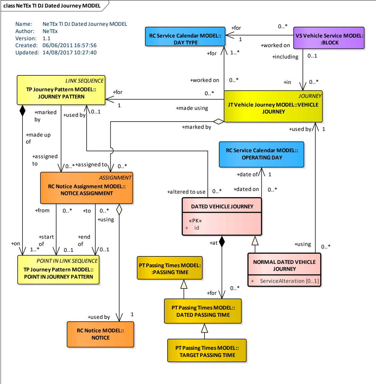
Figure 141 — Dated Journey — Conceptual MODEL (UML)
