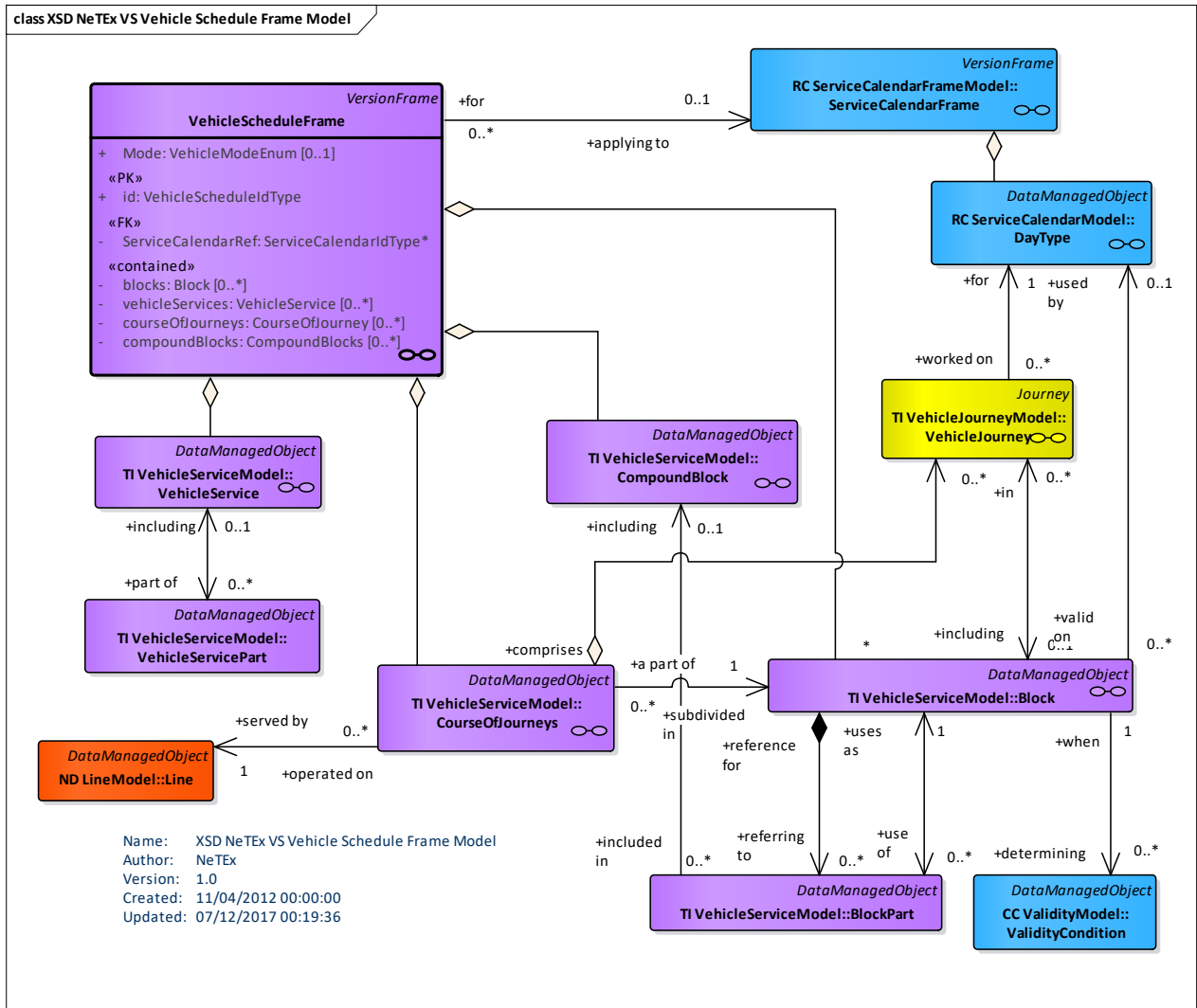
Figure 170 — Vehicle Schedule Frame – Physical Model (UML)
