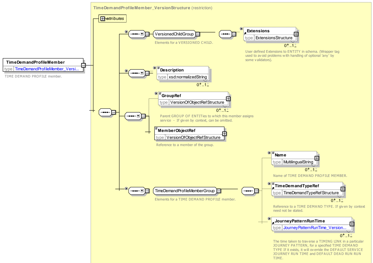
Figure 59 — TimeDemandProfileMember — XSD
