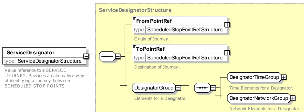
Figure 47 — ServiceDesignator — XSD
