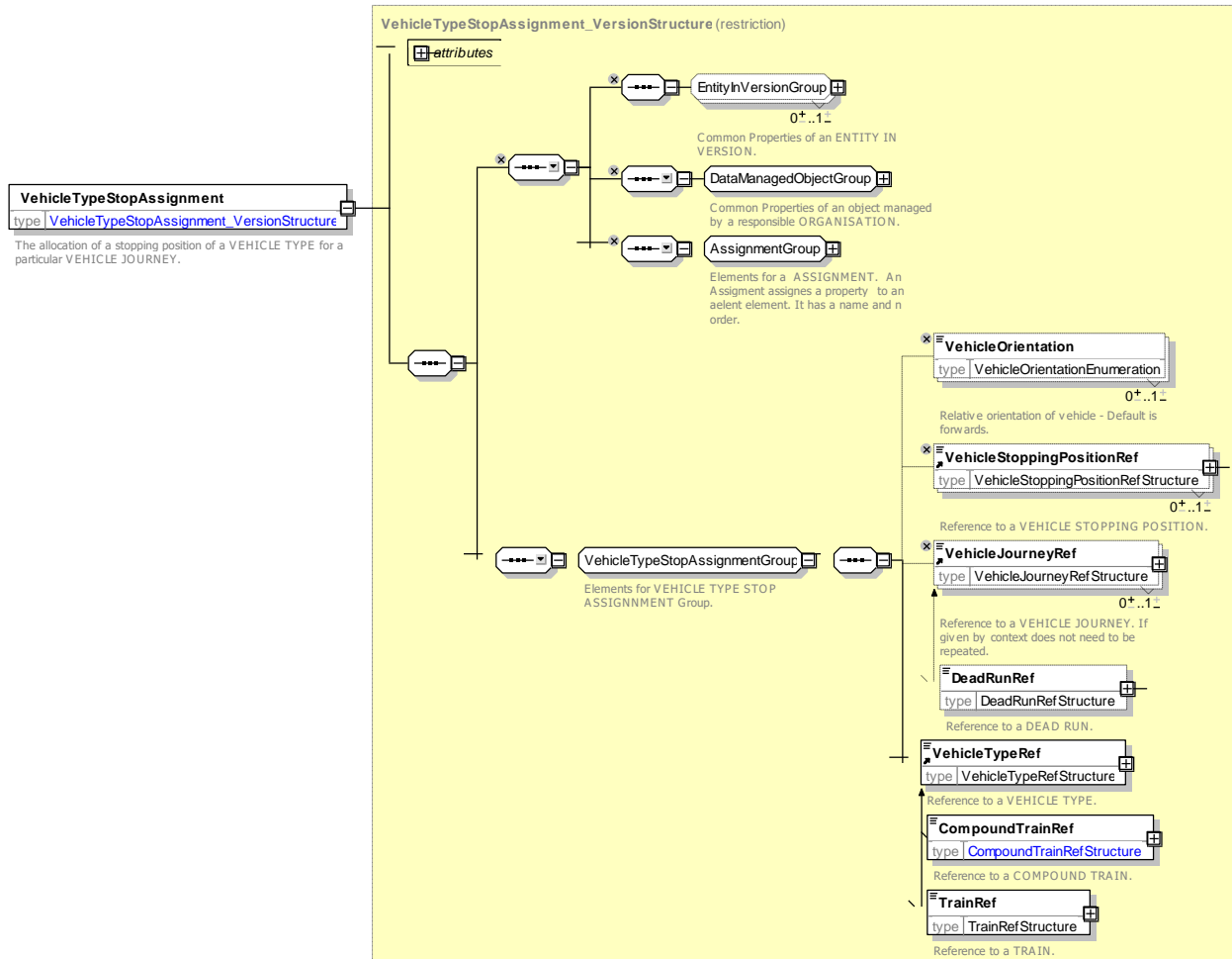
Figure 34 — VehicleTypeStopAssignment — XSD
