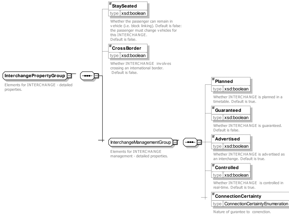
Figure 96 — InterchangePropertyGroup — XSD
