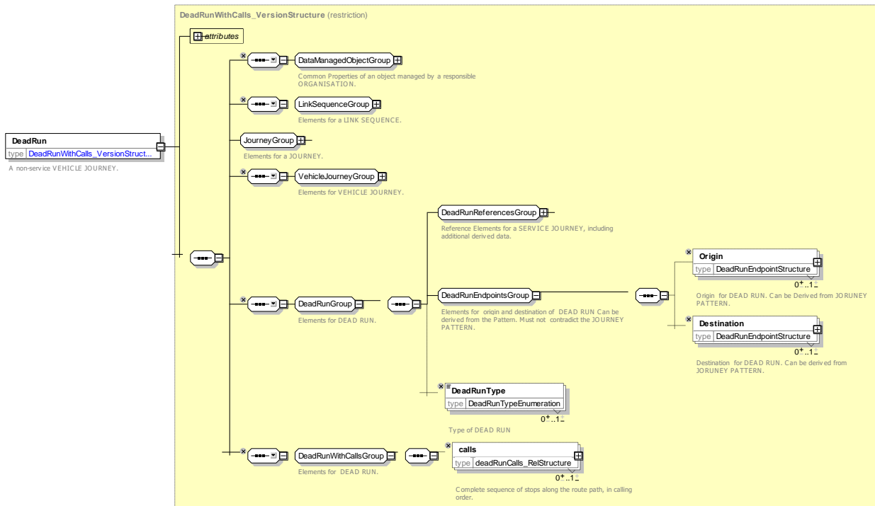
Figure 21 — DeadRun — XSD
