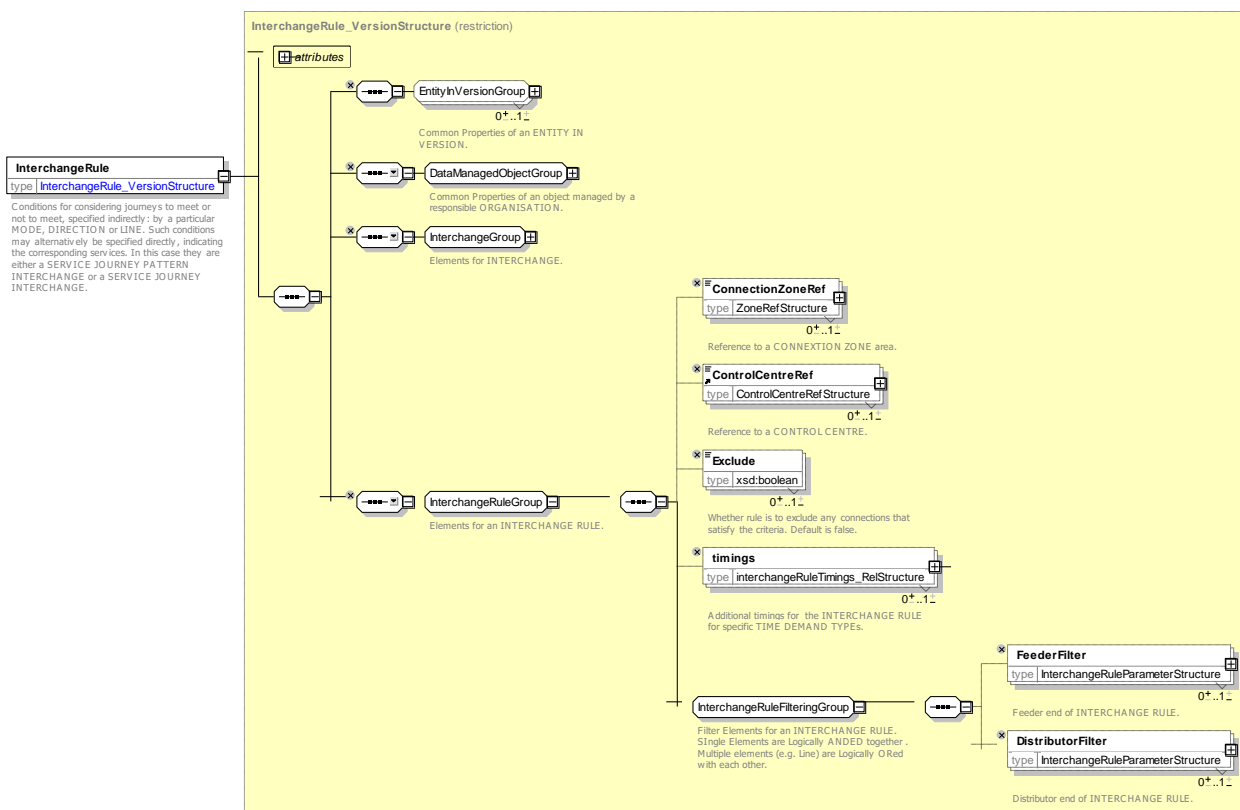
Figure 107 — InterchangeRule — XSD
