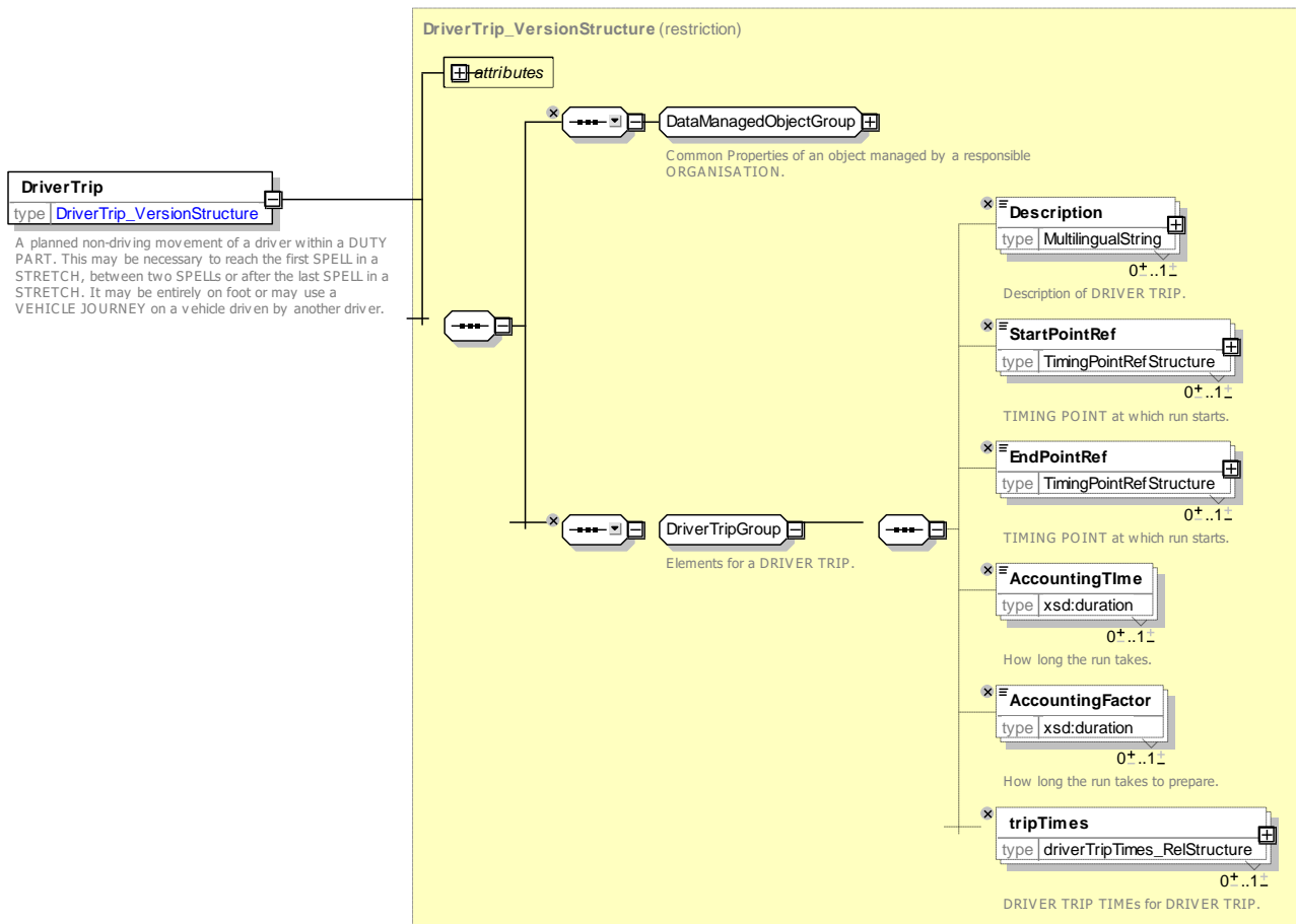
Figure 206 — DriverTrip — XSD
