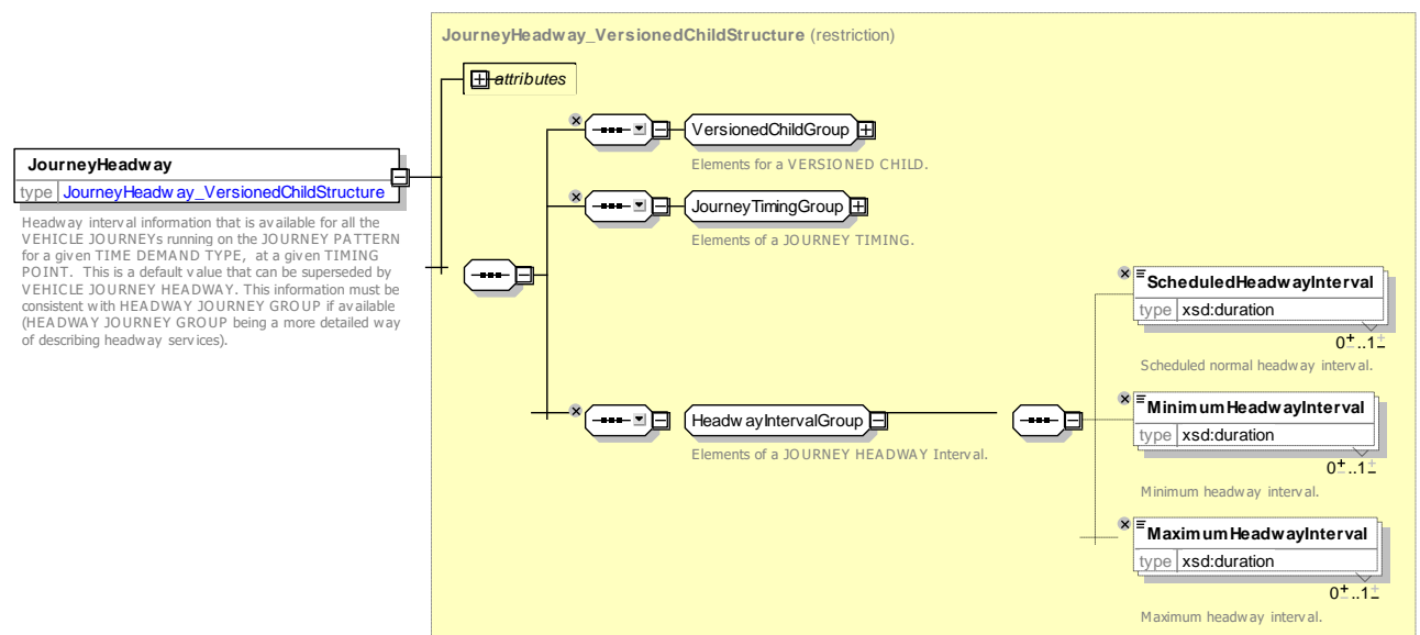
Figure 66 – JourneyHeadway – XSD
