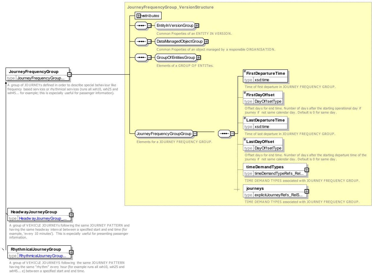
Figure 87 — JourneyFrequencyGroup — XSD
