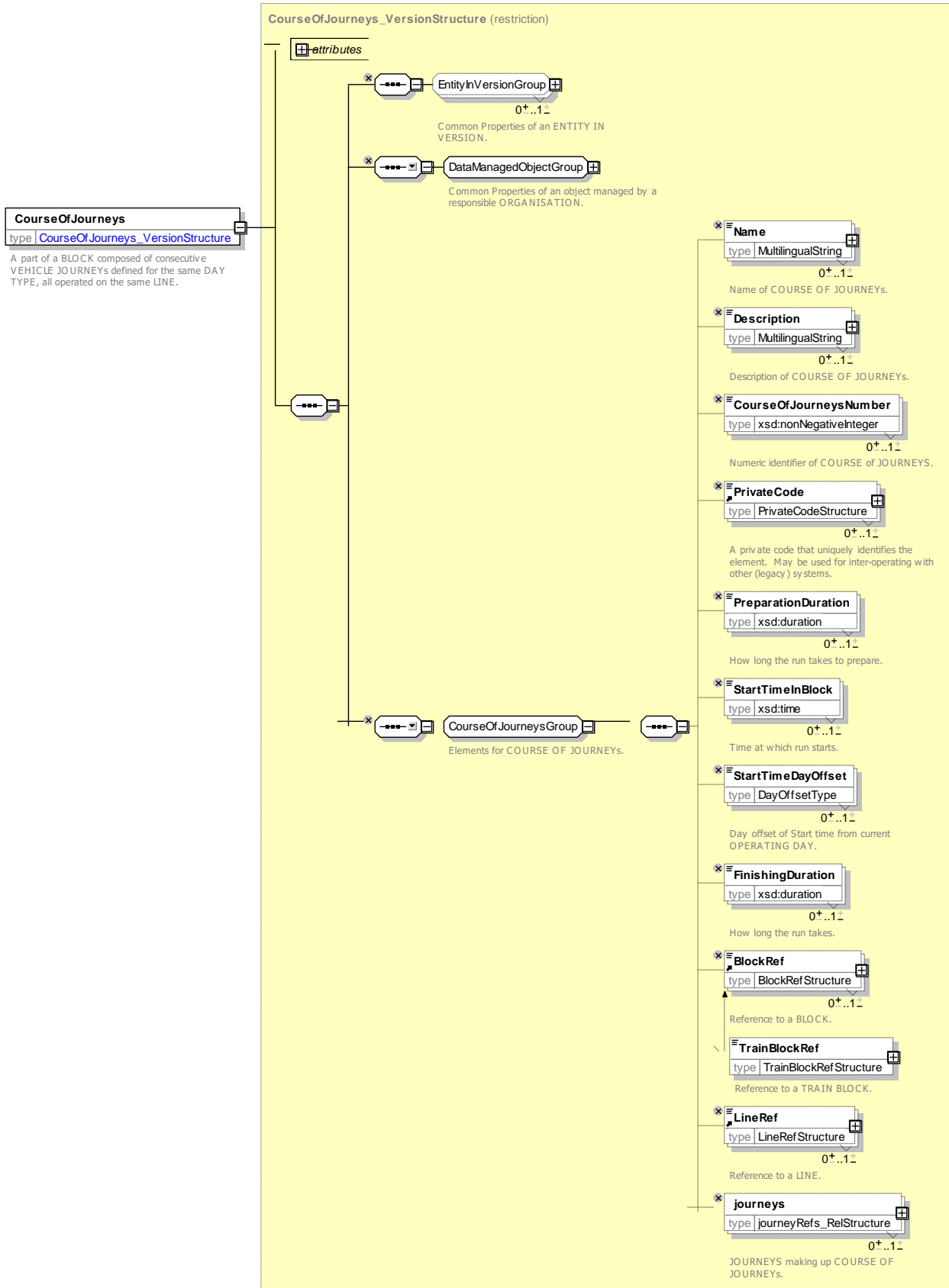
Figure 180 — CourseOfJourneys — XSD
