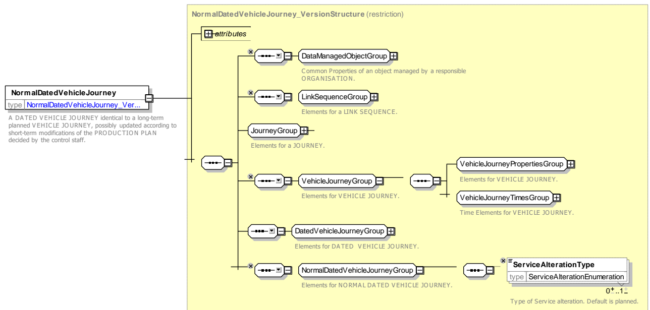
Figure 145 — NormalDatedVehicleJourney — XSD
