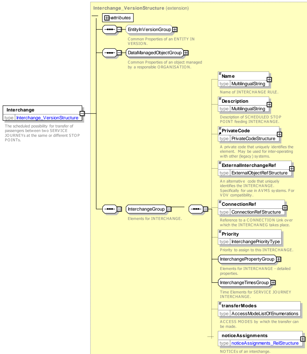
Figure 95 — Interchange — XSD
