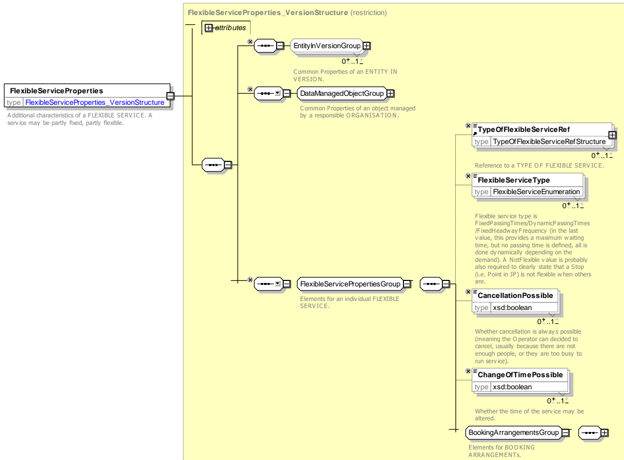
Figure 134 — FlexibleServiceProperties — XSD
