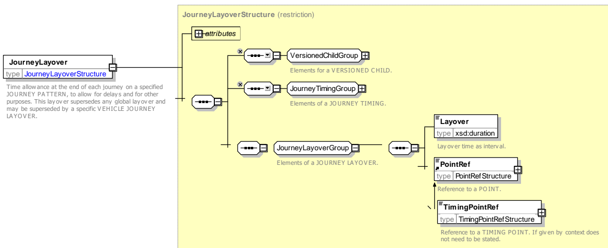
Figure 65 — JourneyLayover — XSD
