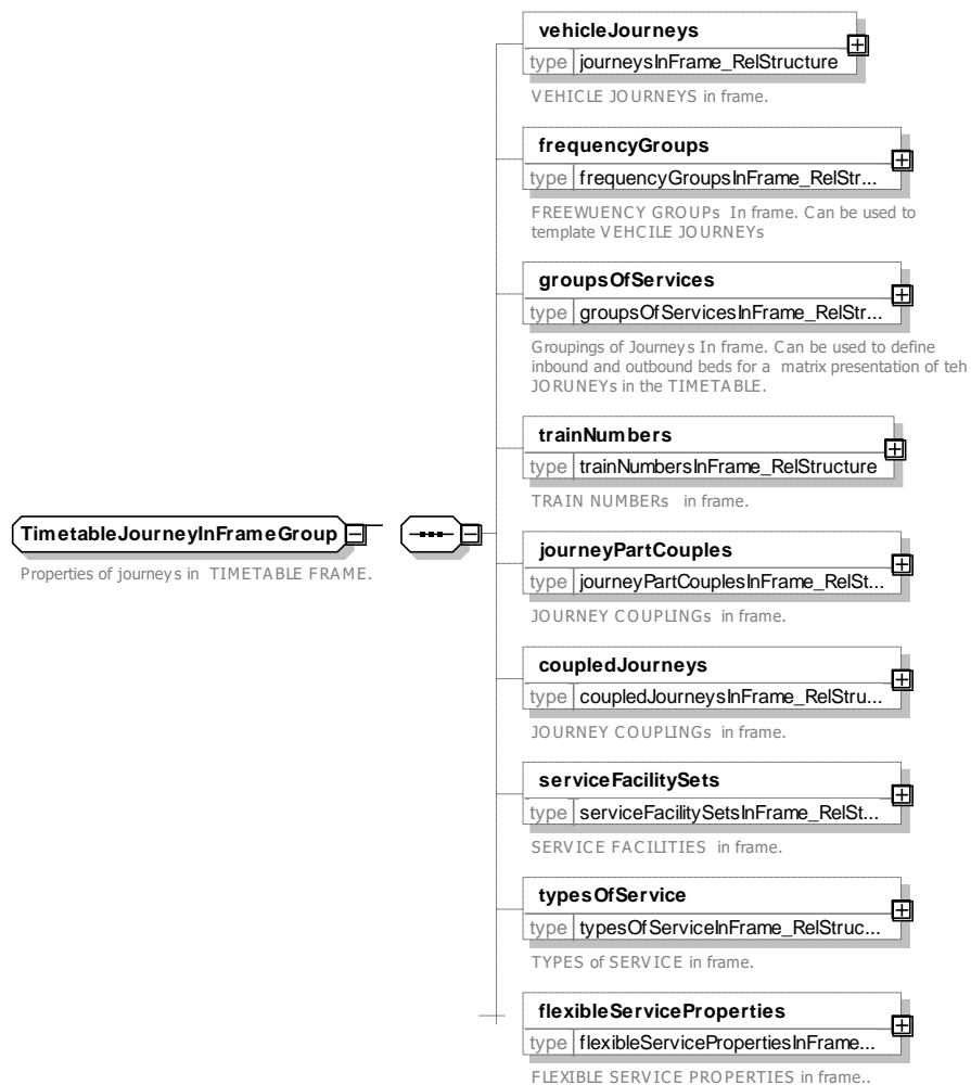
Figure 9 — TimetableJourneyInFrameGroup — XSD
