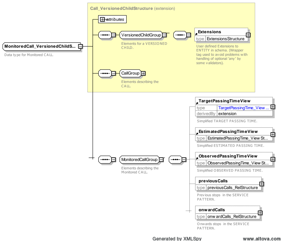
Figure 190 — MonitoredCall — XSD
