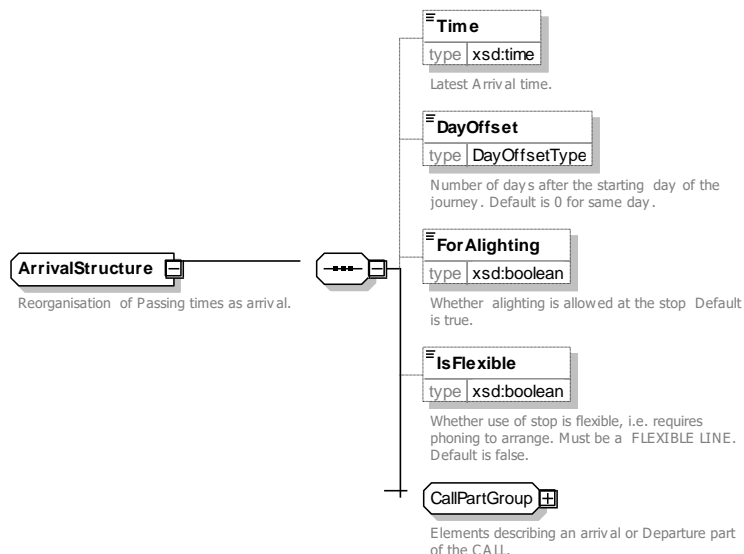
Figure 155 — ArrivalStructure — XSD
