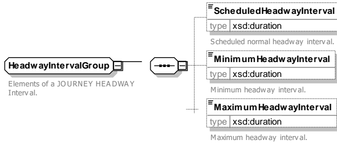
Figure 67 — HeadwayInterval — XSD
