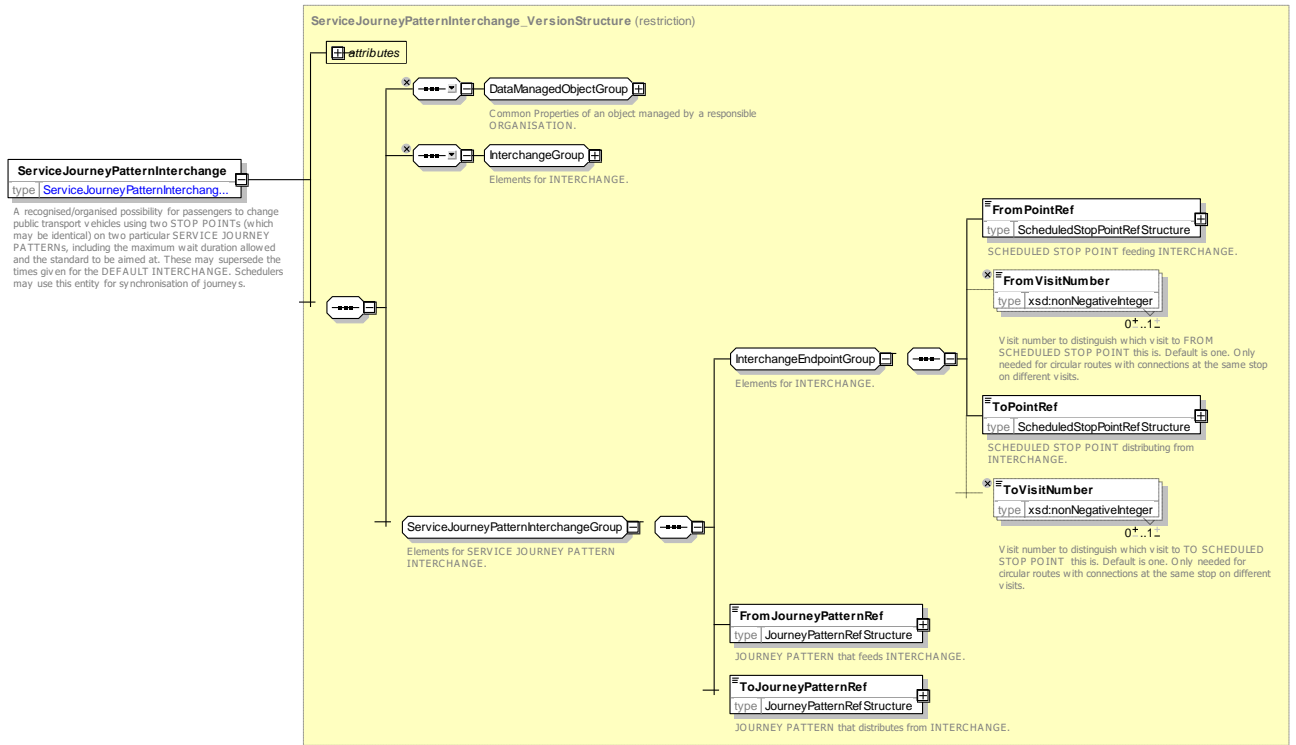
Figure 99 — ServiceJourneyPatternInterchange — XSD
