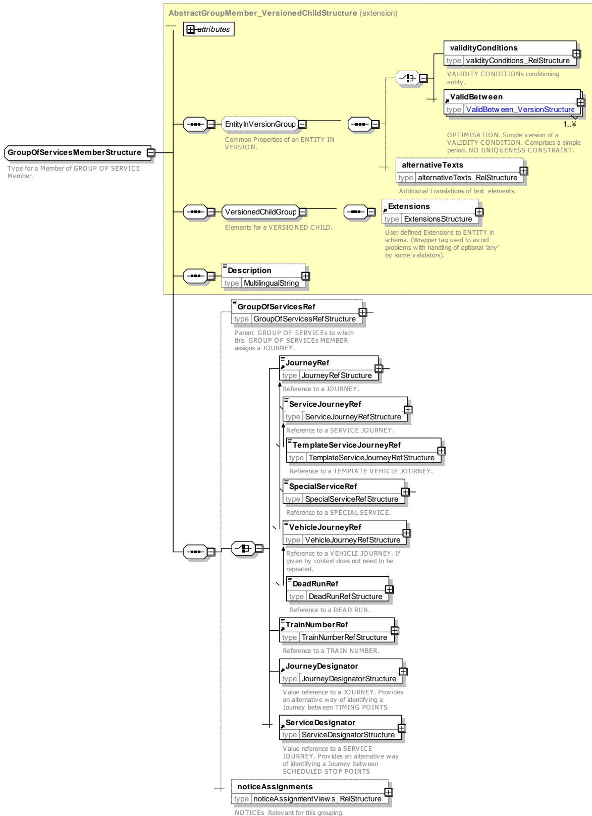
Figure 50 — GroupOfServicesMember — XSD
