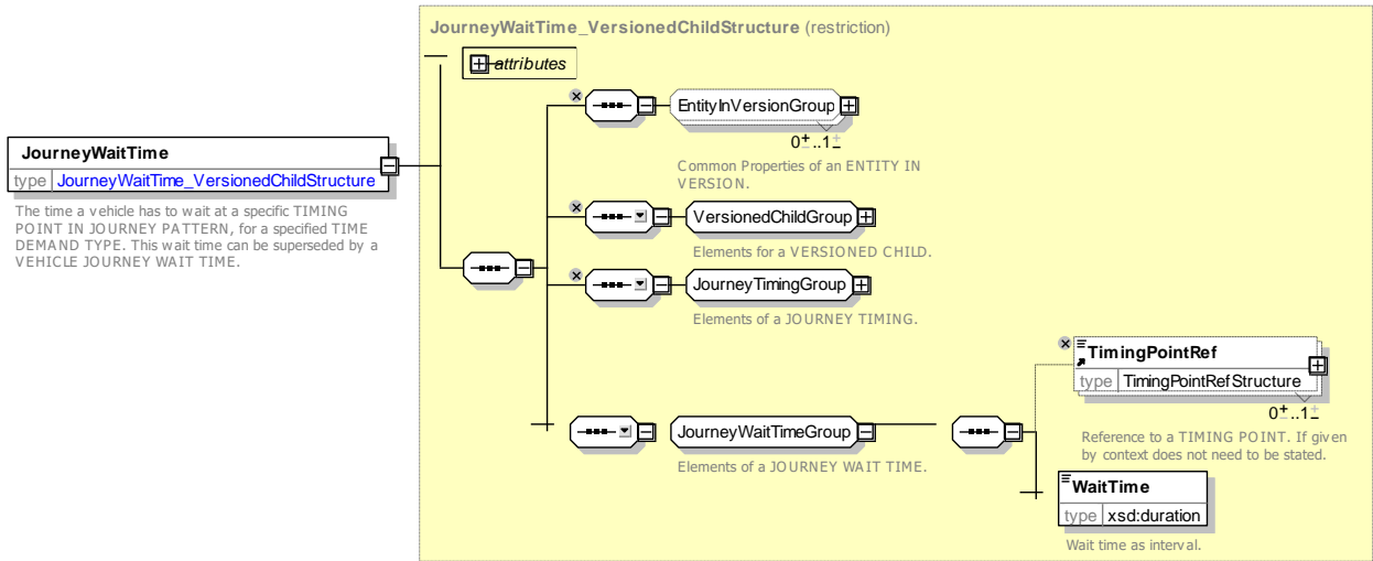
Figure 63 — JourneyWaitTime — XSD
