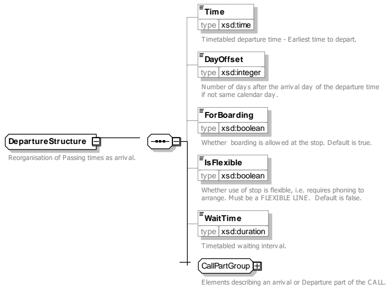
Figure 156 — DepartureStructure — XSD
