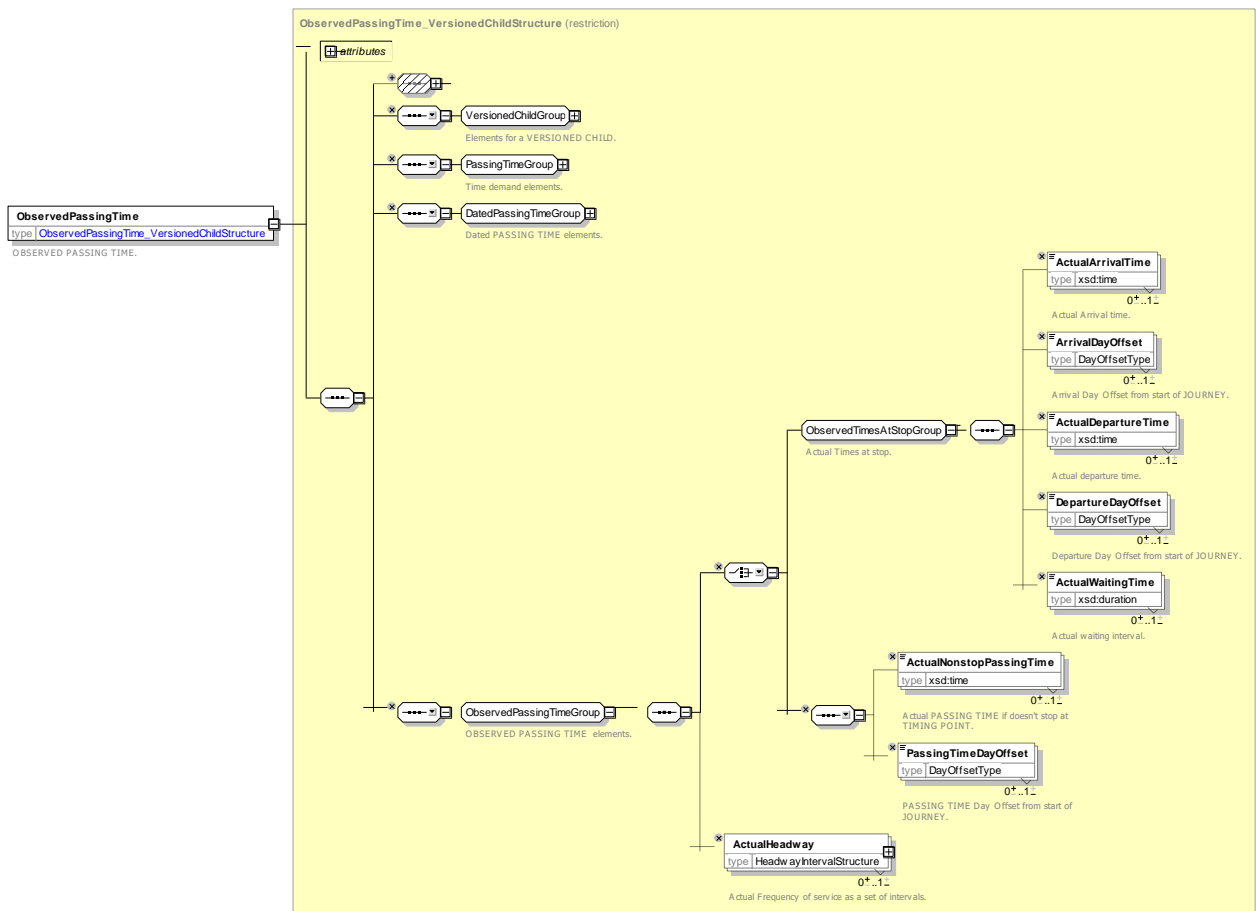
Figure 195 — ObservedPassingTime — XSD
