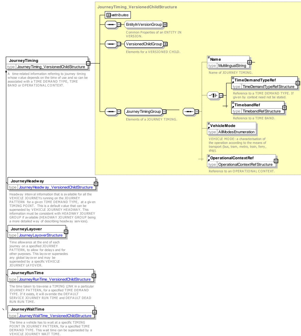
Figure 62 — JourneyTiming — XSD
