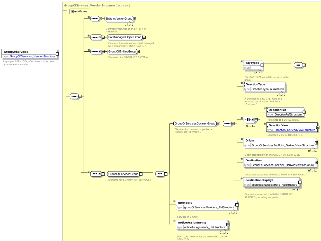
Figure 49 — GroupOfServices — XSD
