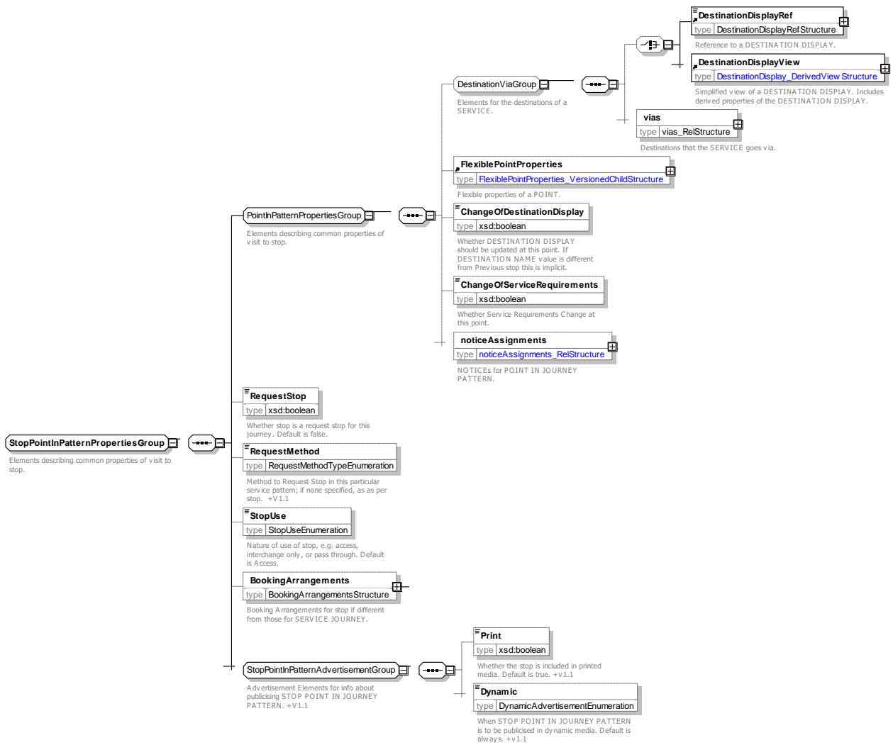
Figure 160 — StopPointInPatternPropertiesGroup — XSD
