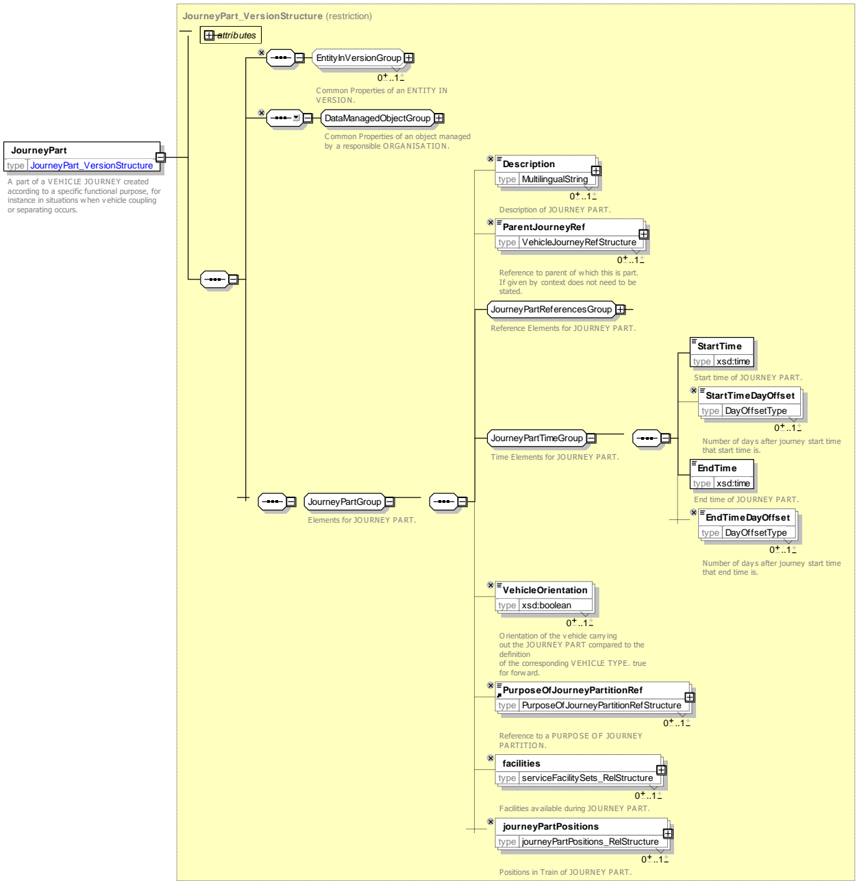
Figure 124 — JourneyPart — XSD
