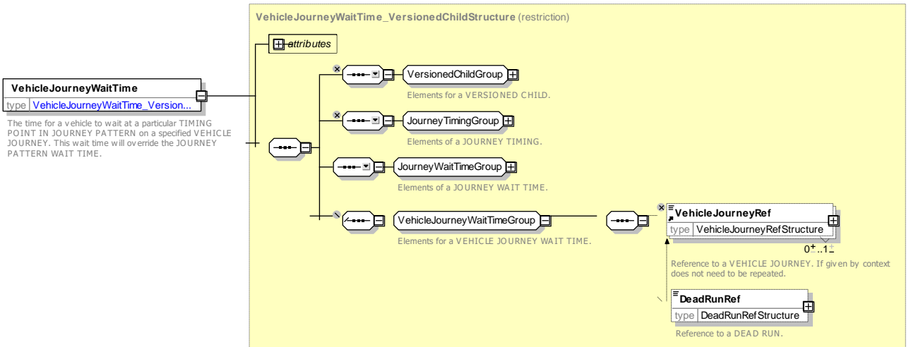
Figure 81 — VehicleJourneyWaitTime — XSD
