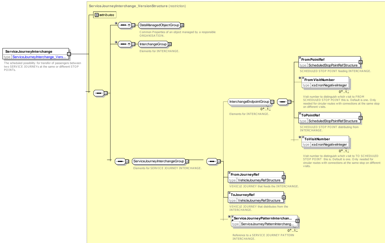
Figure 98 — ServiceJourneyInterchange — XSD
