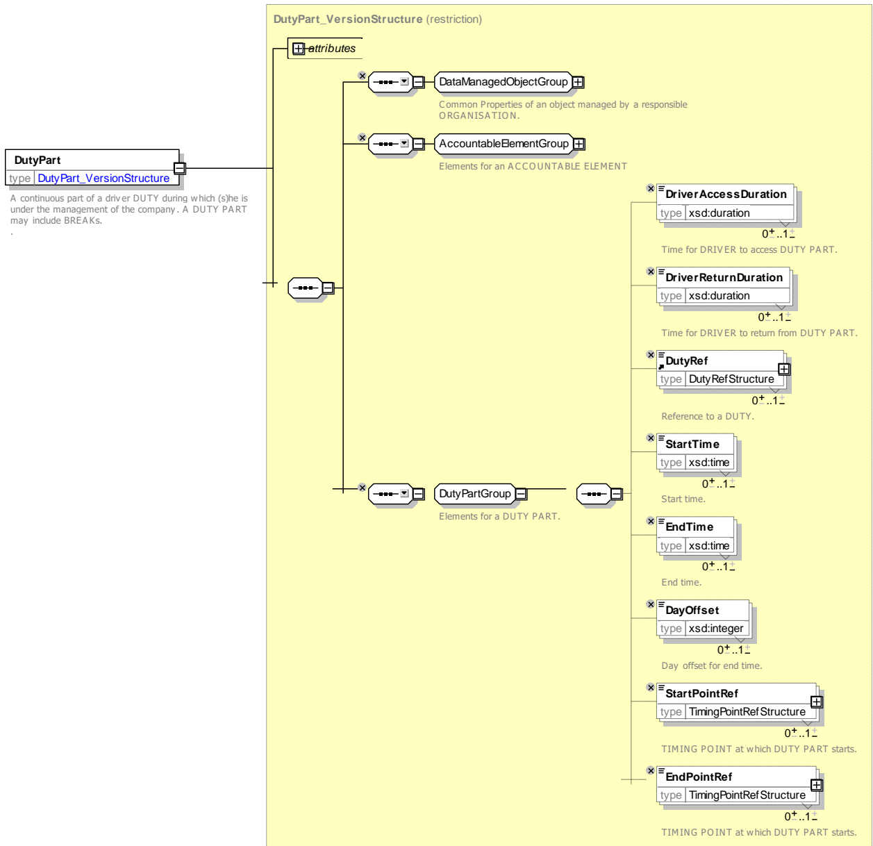
Figure 205 — DutyPart — XSD
