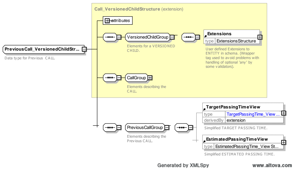
Figure 191 – PreviousCall – XSD
