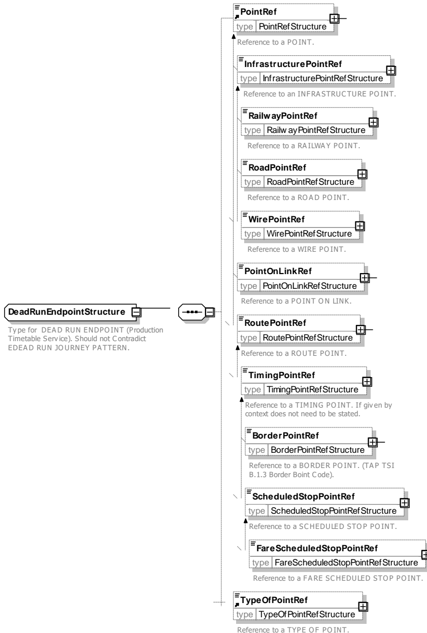
Figure 23 — DeadRunEndPoint — XSD
