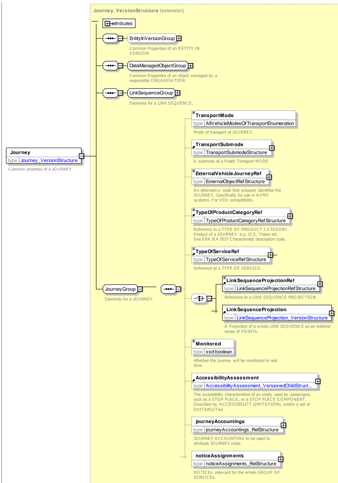
Figure 16 — Journey — XSD
