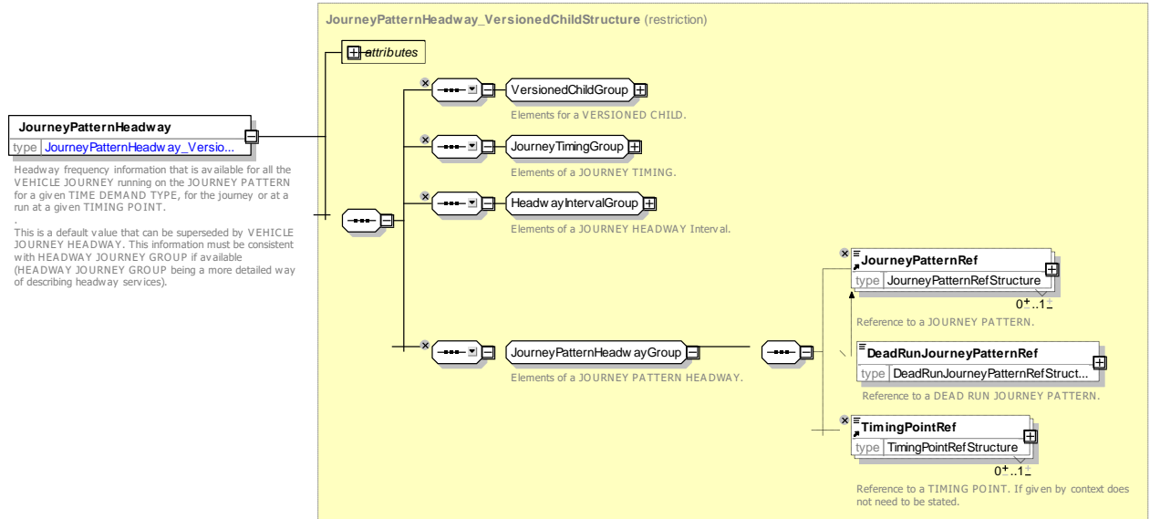
Figure 75 — JourneyPatternHeadway — XSD
