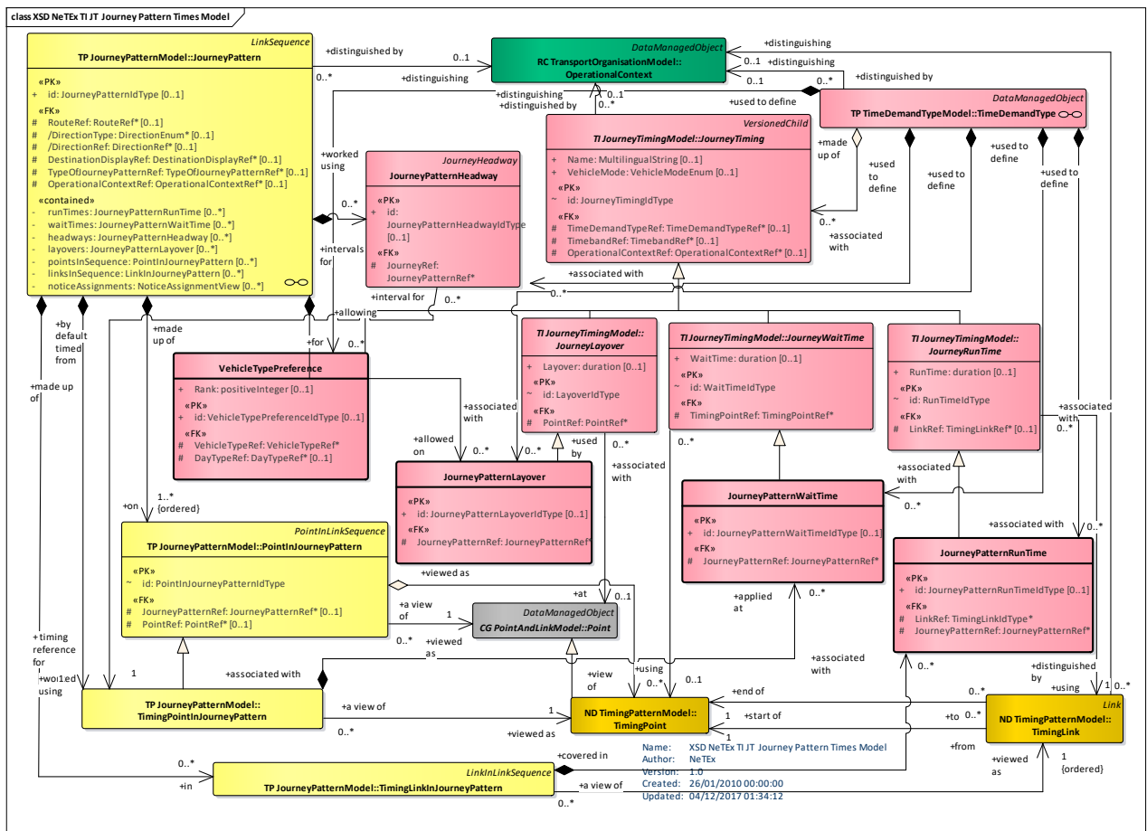
Figure 70 — Journey Pattern Times – Physical Model (UML)
