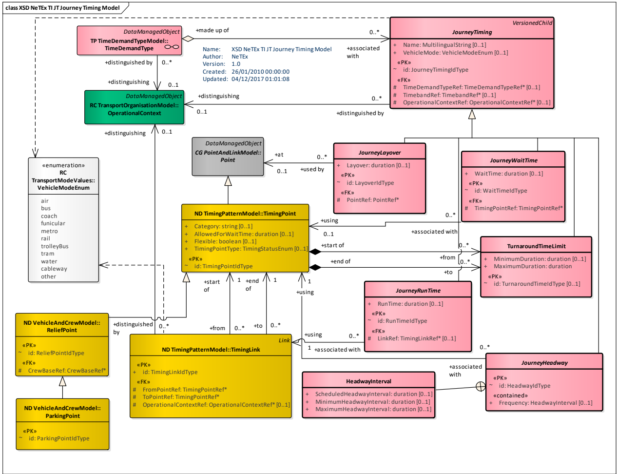
Figure 61 — Journey Timing – Physical Model (UML)
