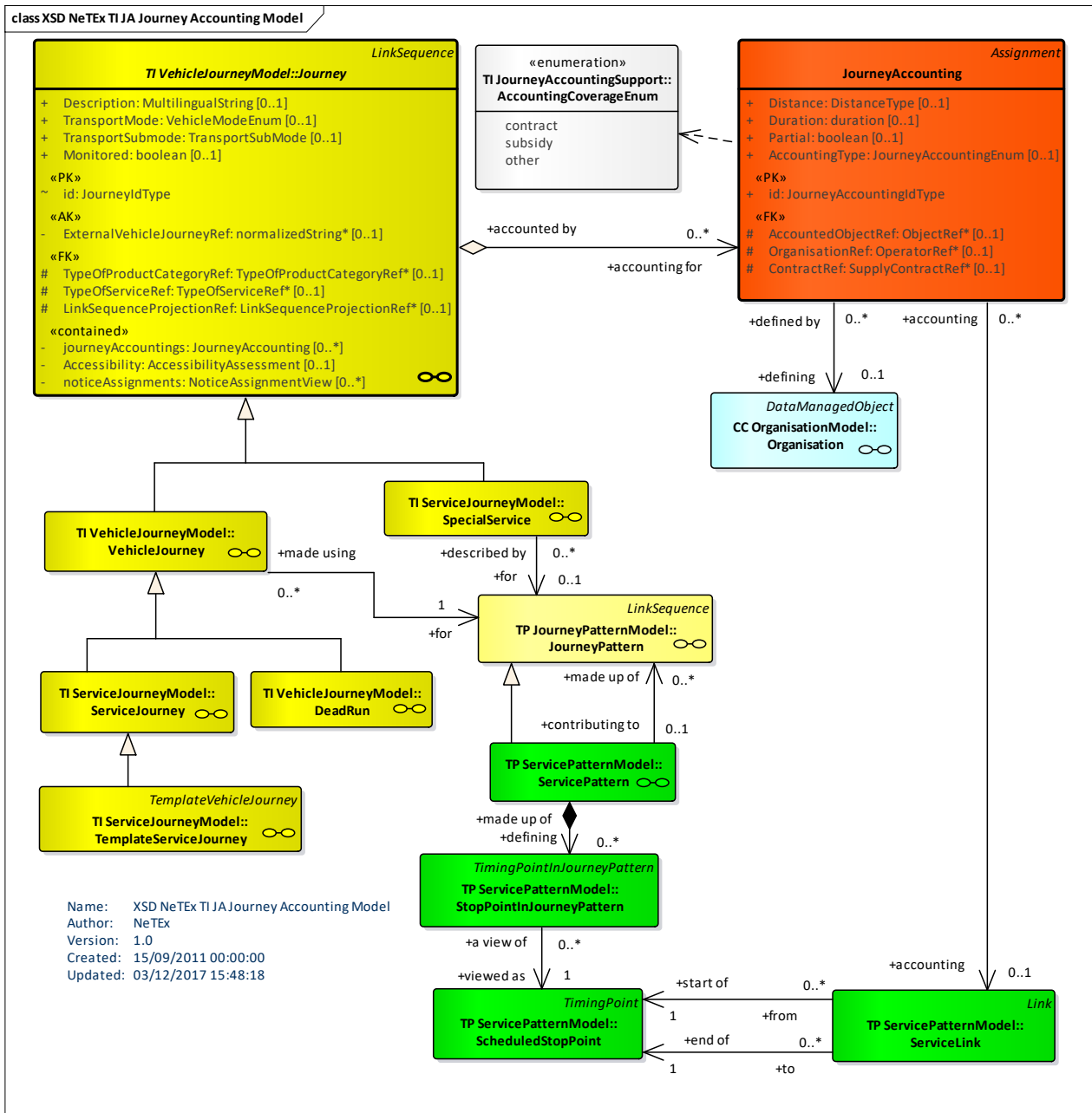
Figure 138 — Journey Accounting – Physical Model (UML)
