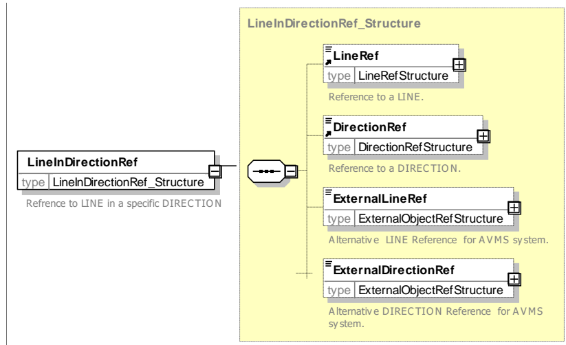
Figure 110 — LineInDirection — XSD
