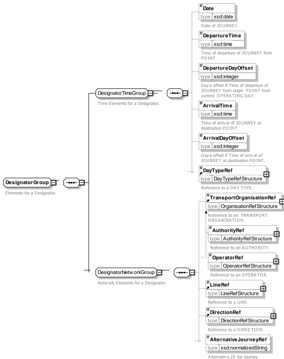
Figure 27 — DesignatorGroup — XSD
