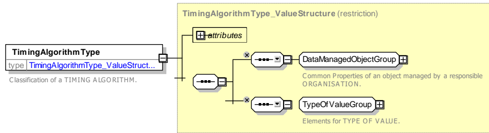
Figure 84 — TimingAlgorithmType — XSD
