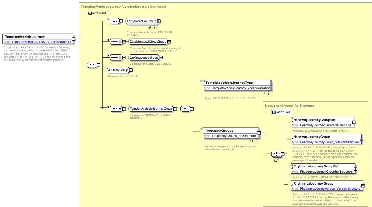
Figure 24 — TemplateVehicleJourney — XSD
