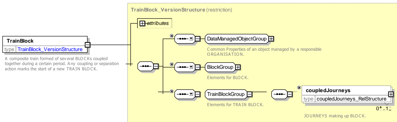
Figure 186 — TrainBlock — XSD
