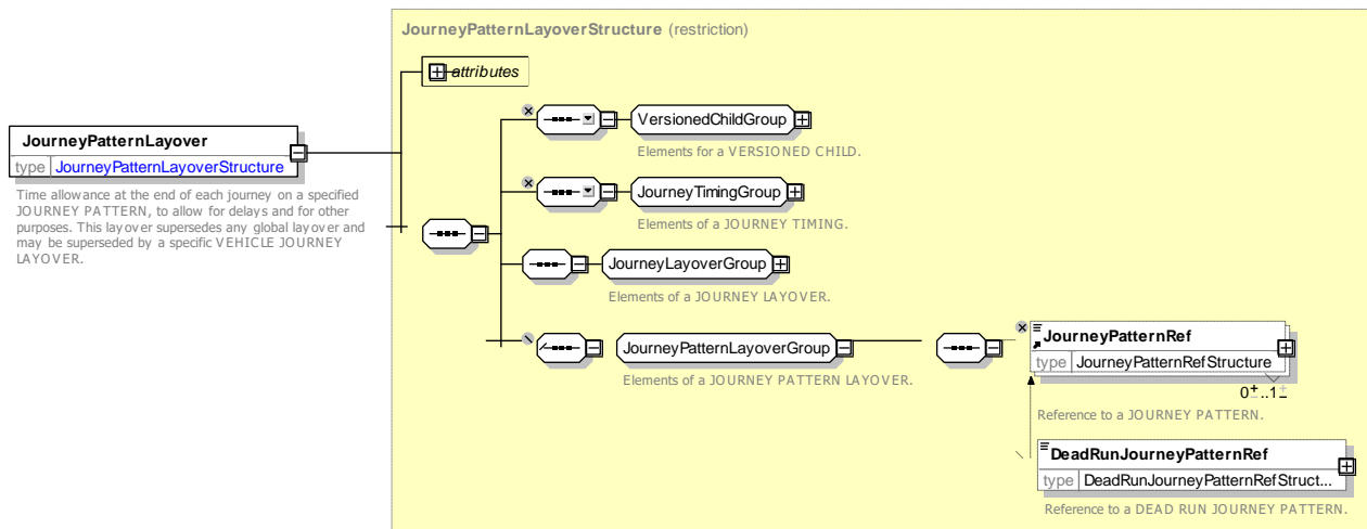
Figure 74 — JourneyPatternLayover — XSD
