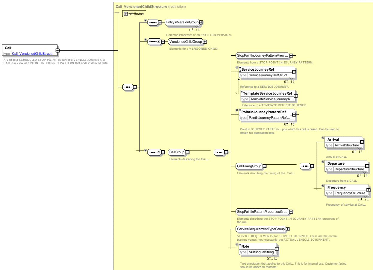
Figure 153 — Call — XSD
