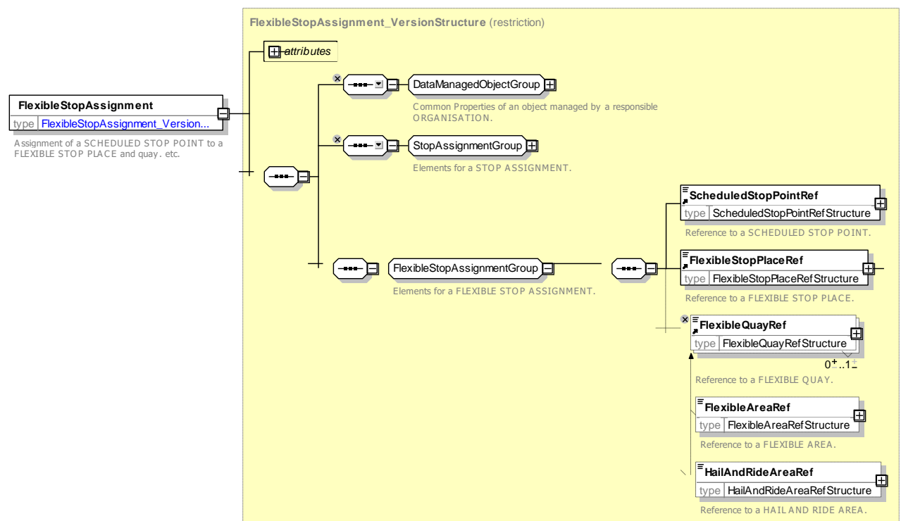
Figure 135 — FlexibleStopAssignment — XSD
