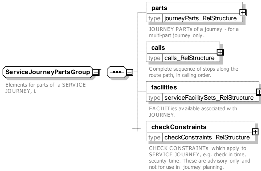
Figure 43 — ServiceJourneyPartsGroup — XSD
