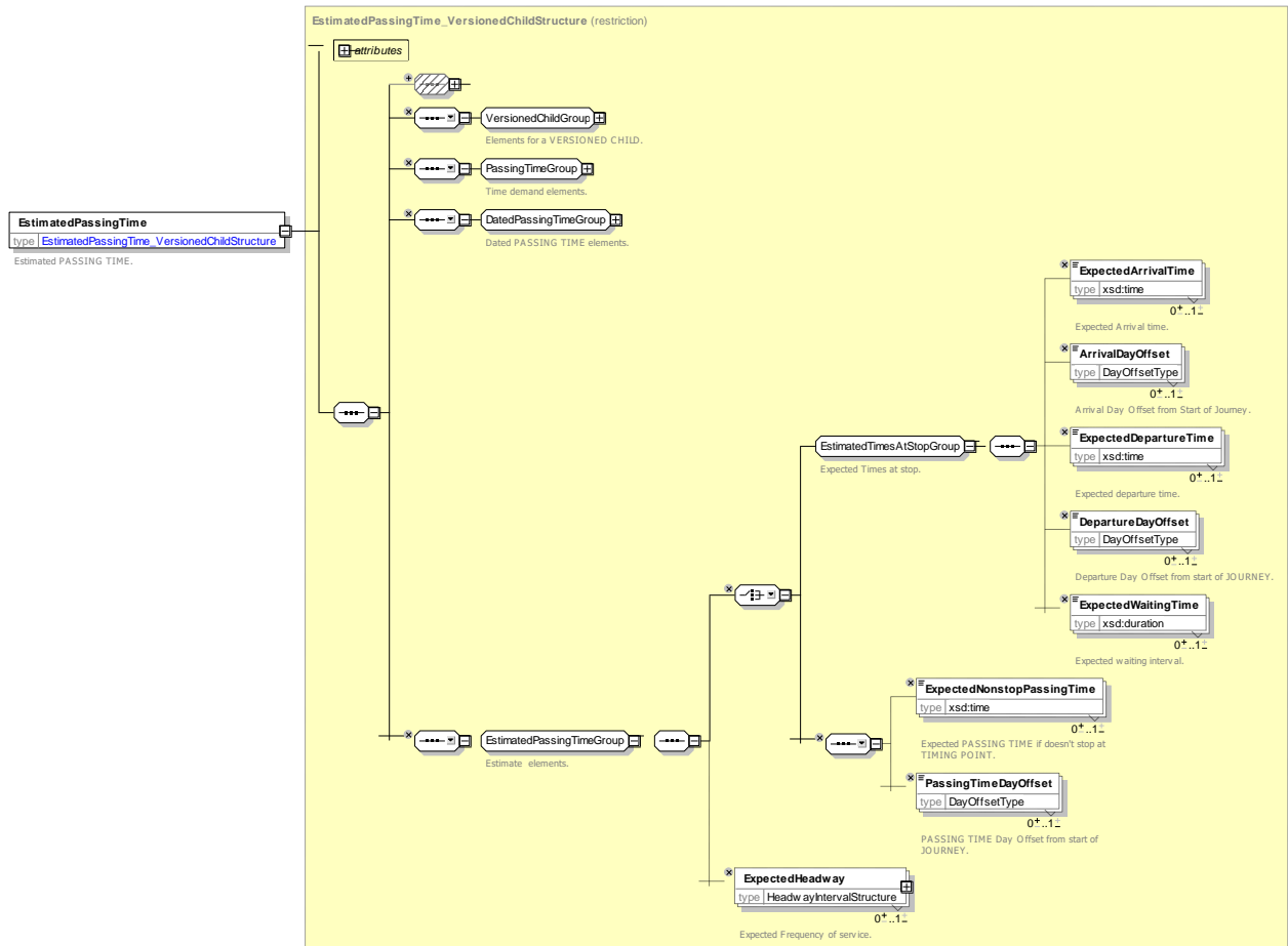
Figure 194 — EstimatedPassingTime — XSD
