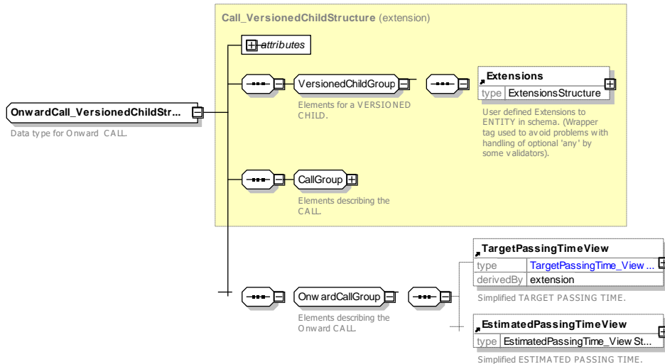
Figure 192 — OnwardCall — XSD
