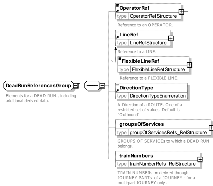
Figure 22 — DeadRunReferencesGroup — XSD
