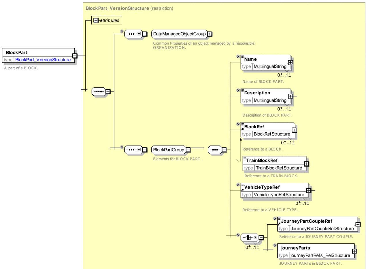
Figure 178 — BlockPart — XSD
