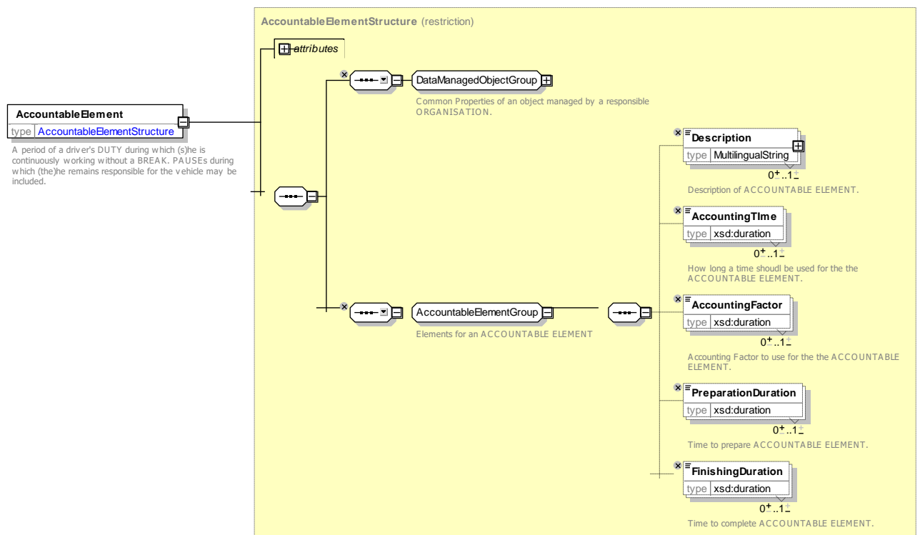
Figure 204 — AccountableElement — XSD
