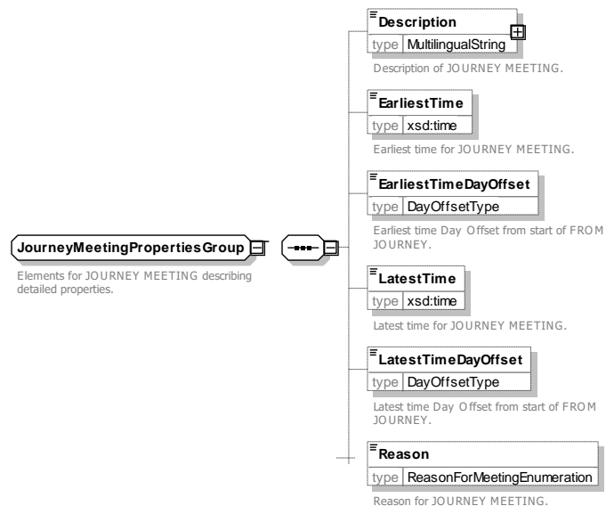
Figure 101 — JourneyMeetingPropertiesGroup — XSD
