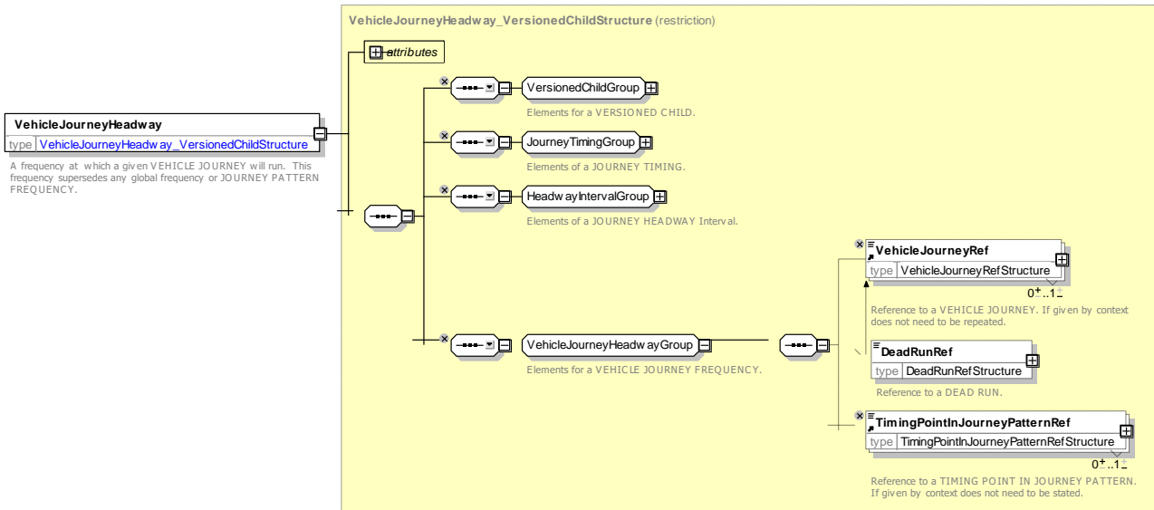
Figure 90 — VehicleJourneyHeadway — XSD
