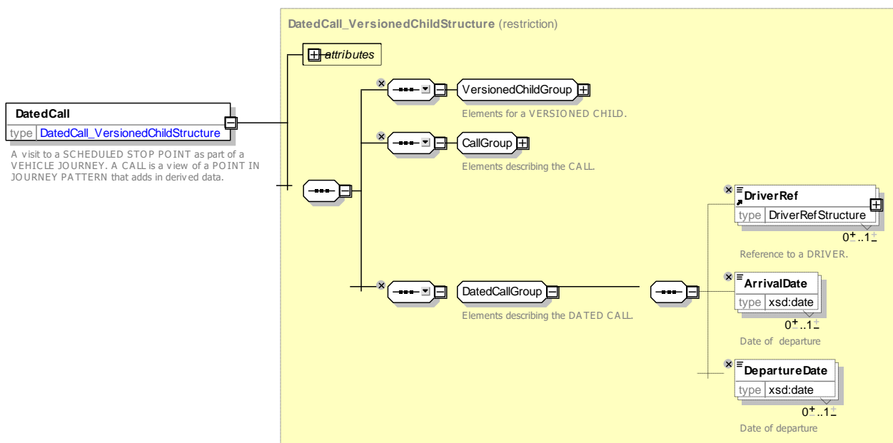
Figure 166 — DatedCall — XSD
