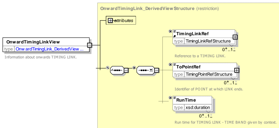
Figure 158 — OnwardTimingLinkView — XSD
