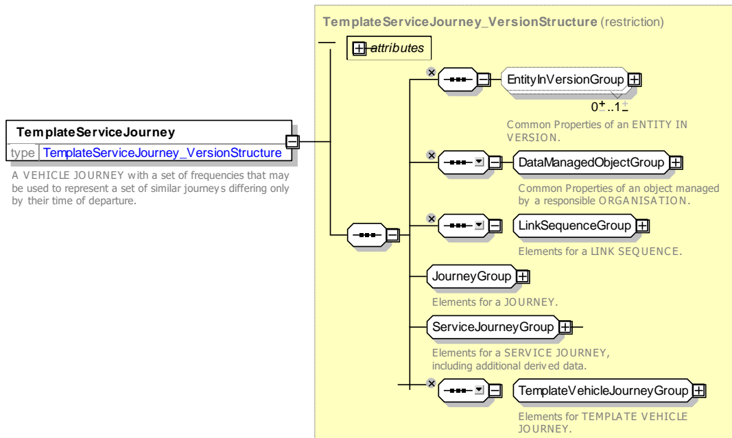
Figure 48 — TemplateServiceJourney — XSD
