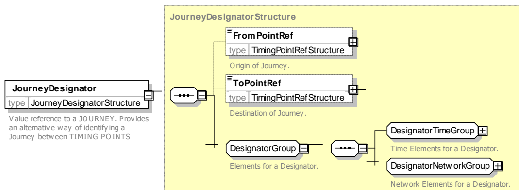
Figure 26 — JourneyDesignator — XSD
