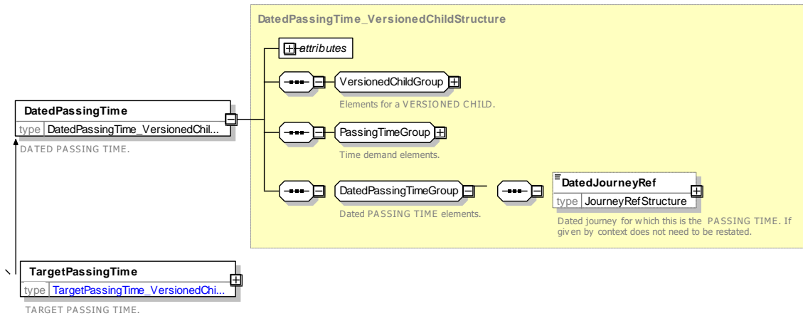
Figure 150 — DatedPassingTime — XSD
