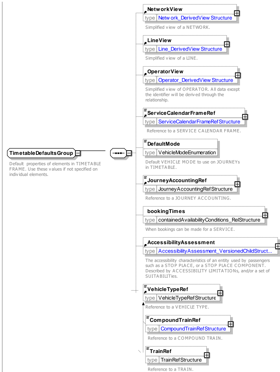
Figure 8 — TimetableDefaultsGroup — XSD
