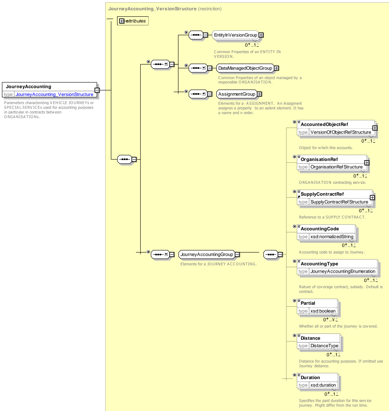
Figure 139 — JourneyAccounting — XSD
