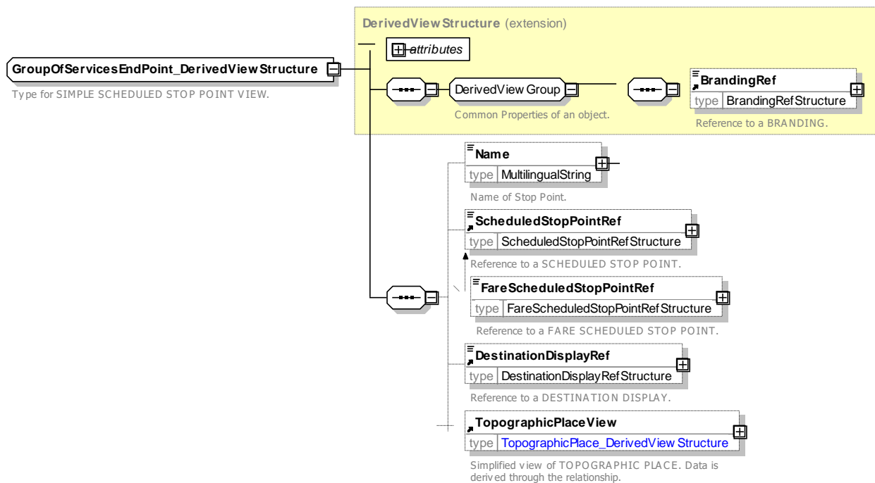
Figure 51 — GroupOfServicesEndPointView — XSD
