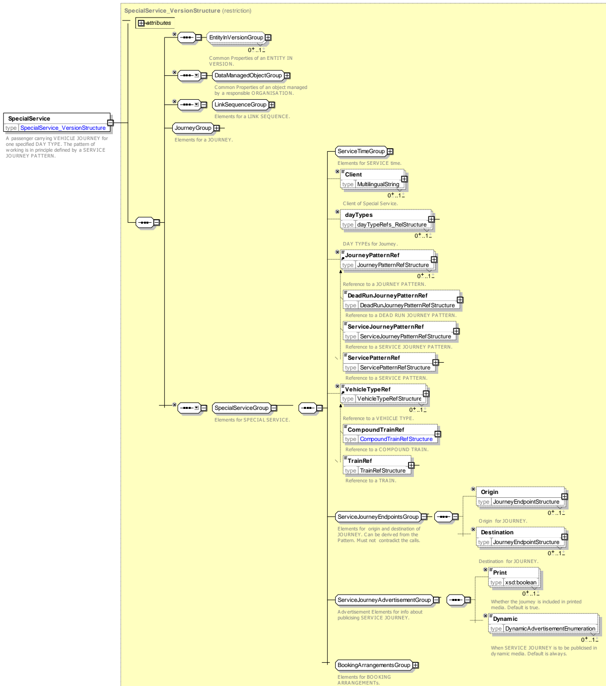
Figure 45 — SpecialService — XSD
