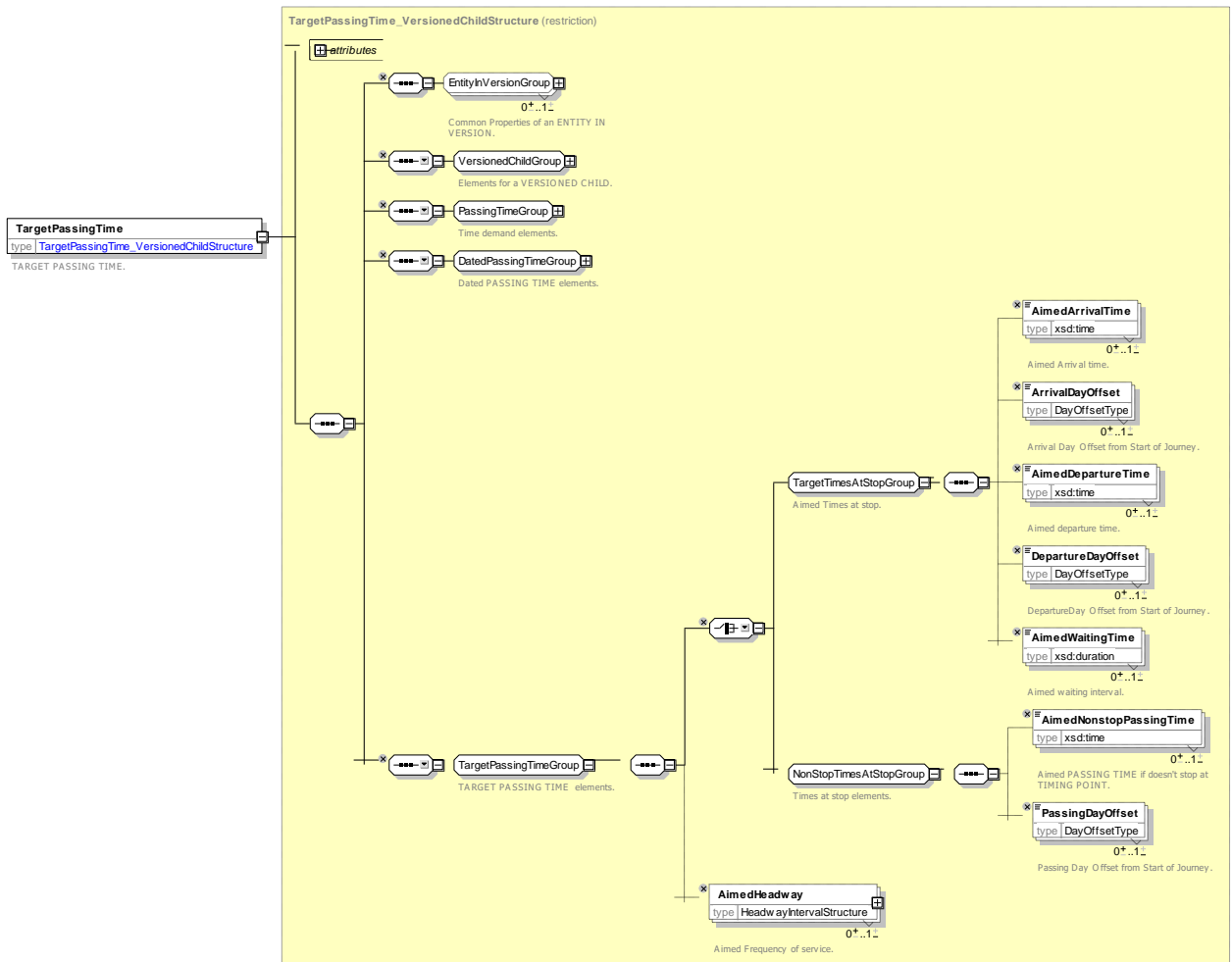
Figure 196 — TargetPassingTime — XSD
