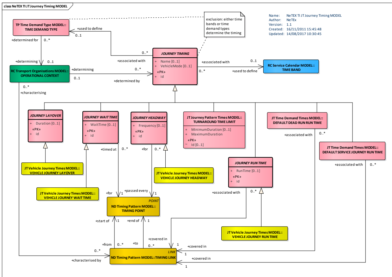
Figure 60 — Journey Timing – Conceptual MODEL (UML)
