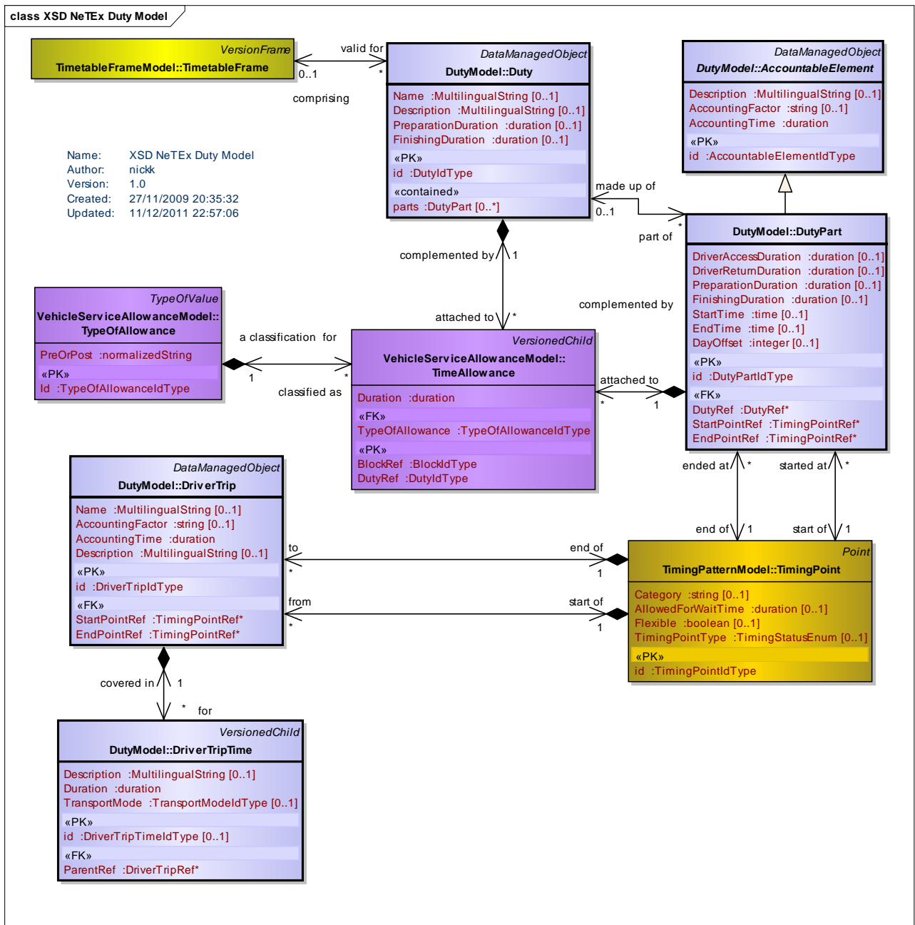
Figure 202 — Duty – Physical Model (UML)
